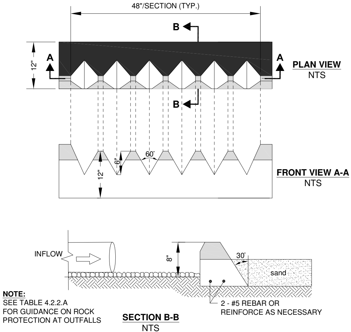
FIGURE 6.2.6.C FLOW SPREADER OPTION C: NOTCHED CURB SPREADER
