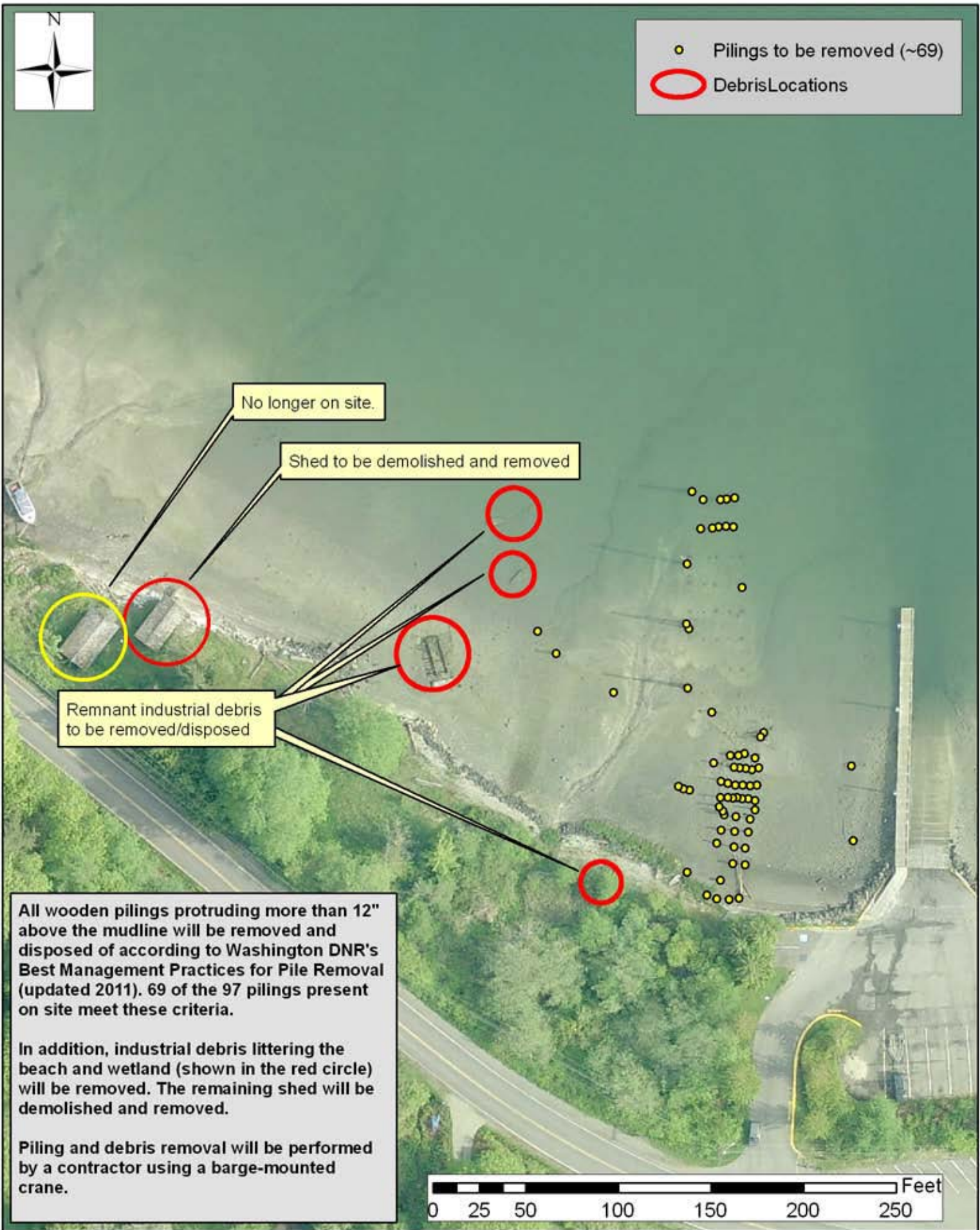
Figure 2: Phase 1--Piling/Debris Removal Dockton Shoreline Restoration Project
