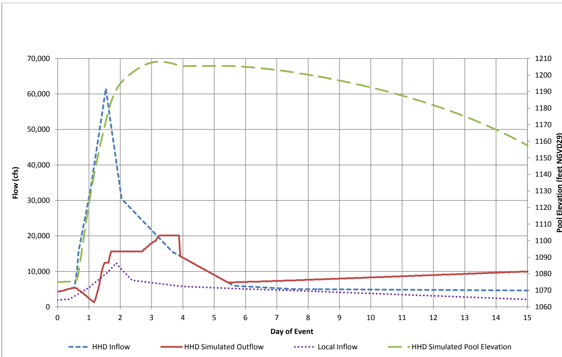
Figure 22 – Simulated Howard Hanson Dam Operations, 0.2 Percent Flood, Upper Confidence Limit (5%)
