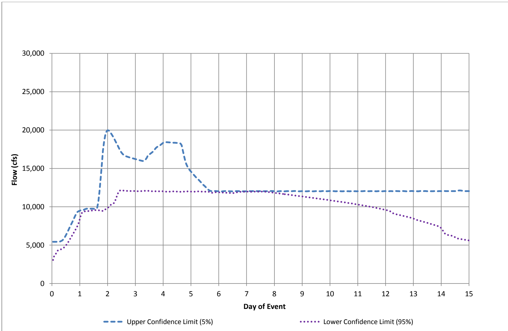
Figure 33 – Green River at Auburn Simulated Discharge, 0.5 Percent Flood
