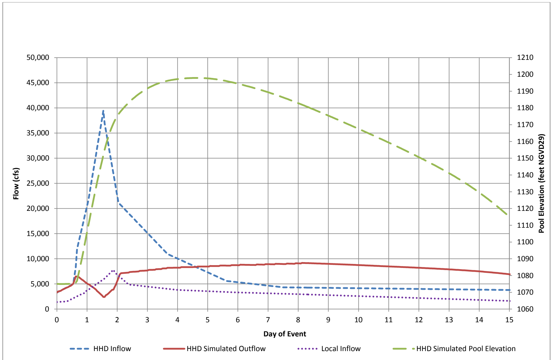
Figure 20 - Simulated Howard Hanson Dam Operations, 0.2 Percent Flood, Lower Confidence Limit (95%)
