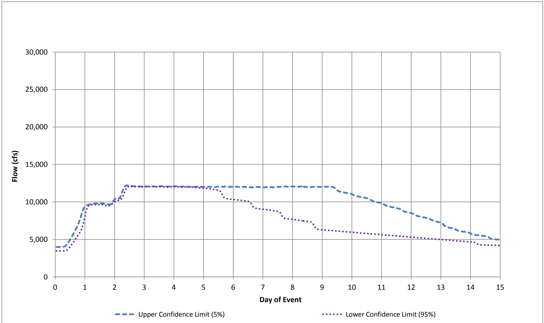
Figure 27 – Green River at Auburn Simulated Discharge, 4 Percent Flood
