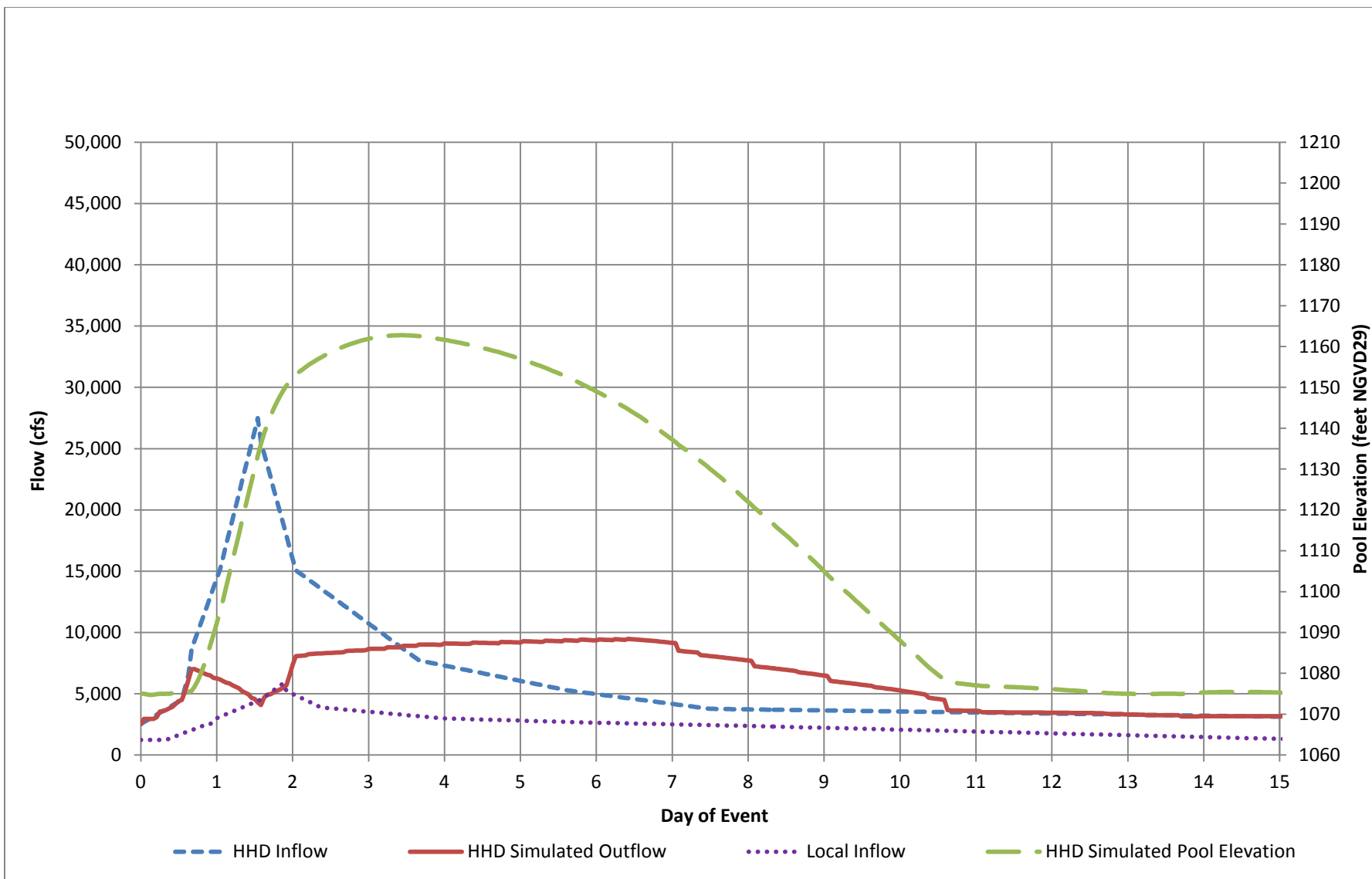
Figure 11 – Simulated Howard Hanson Dam Operations, 2 Percent Flood, Lower Confidence Limit (95%)
