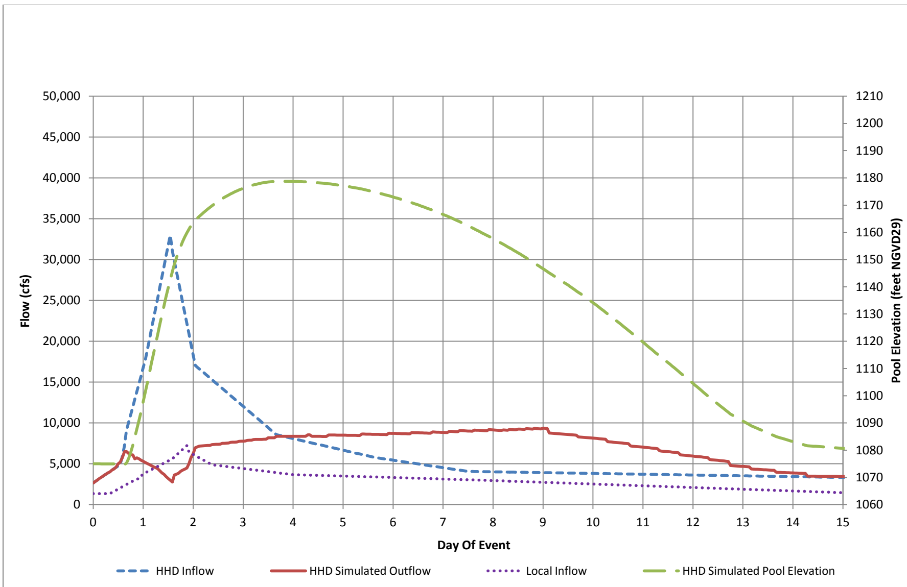
Figure 10 – Simulated Howard Hanson Dam Operations, 4 Percent Flood, Upper Confidence Limit (5%)
