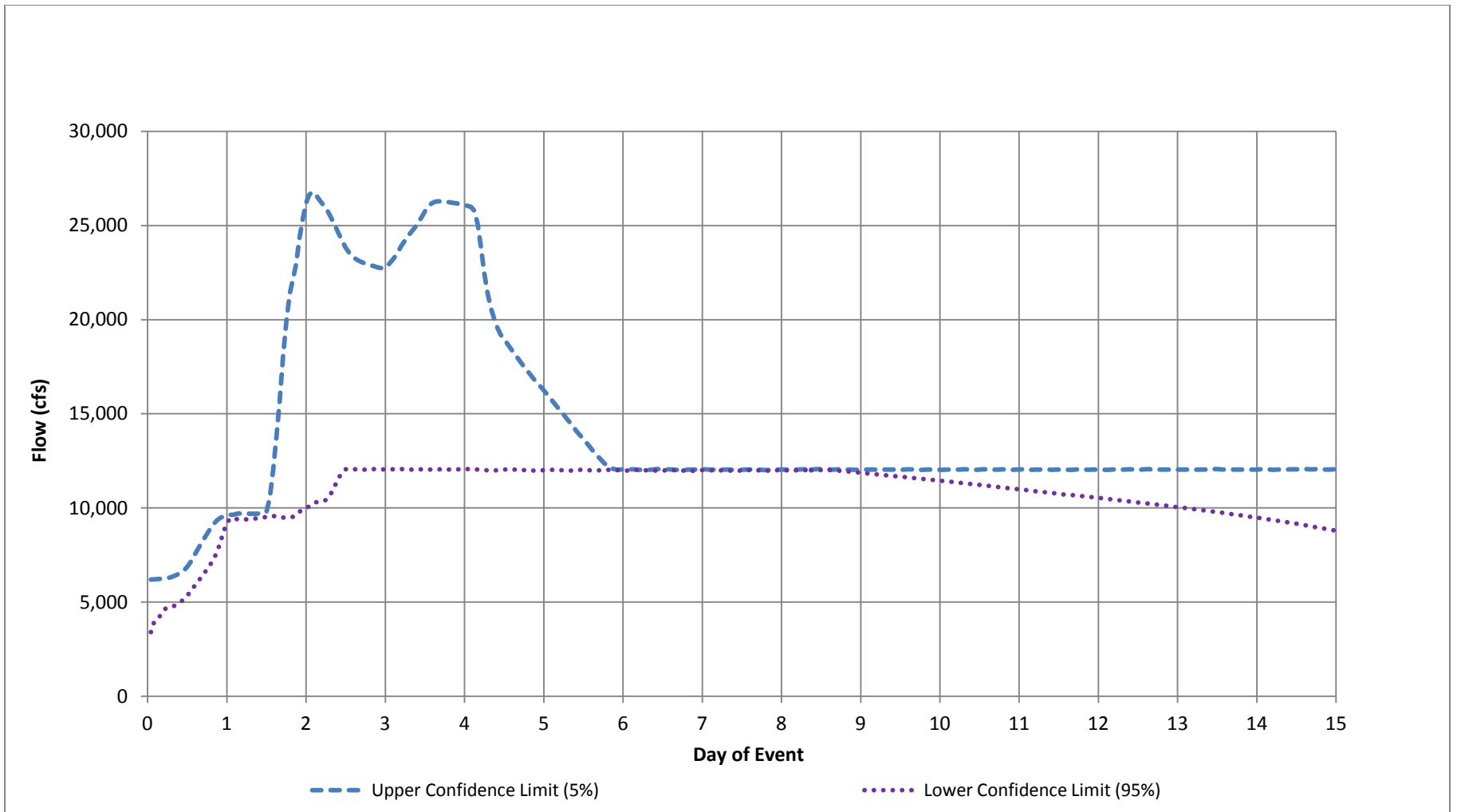
Figure 35 – Green River at Auburn Simulated Discharge, 0.2 Percent Flood
