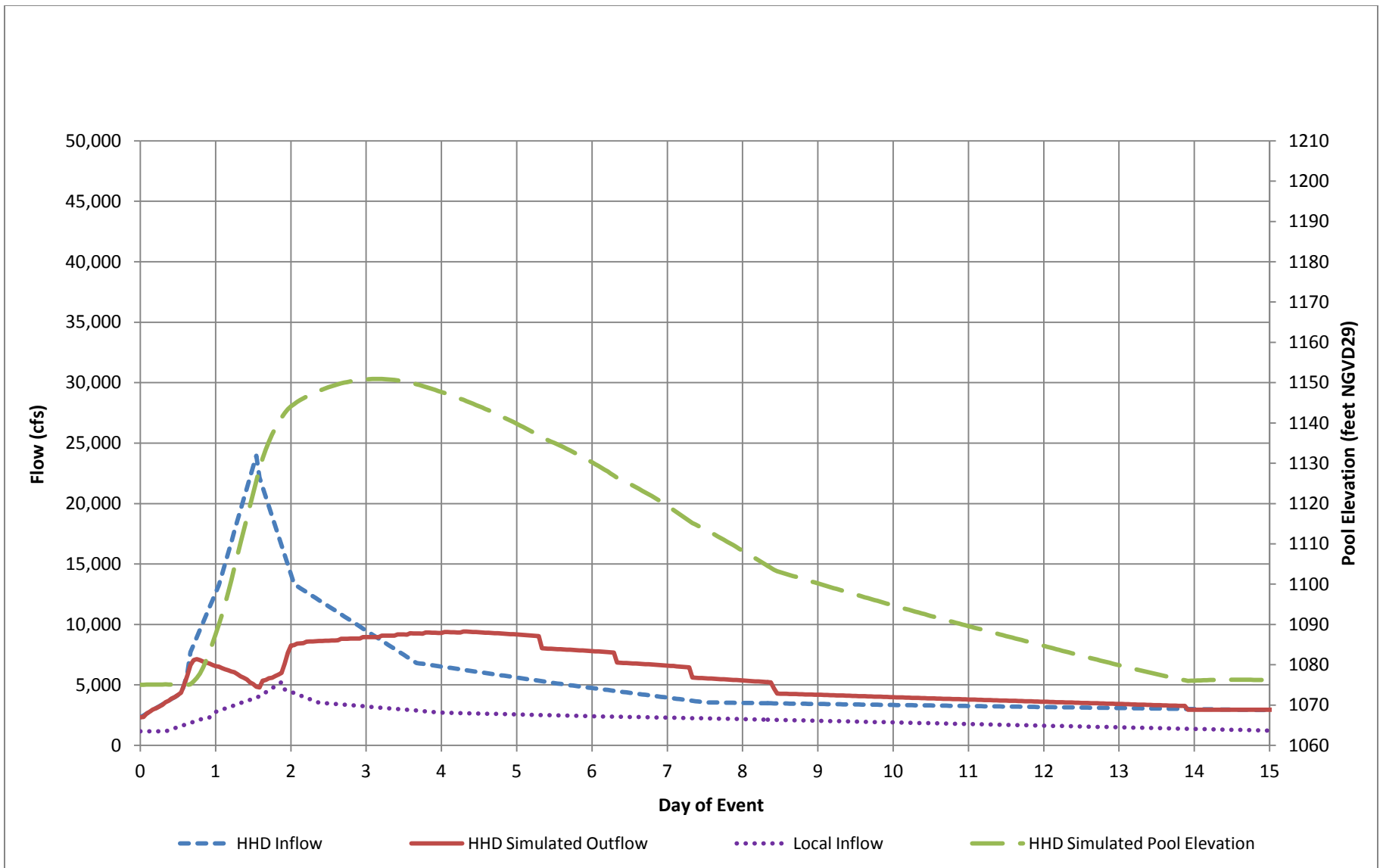
Figure 8 – Simulated Howard Hanson Dam Operations, 4 Percent Flood, Lower Confidence Limit (95%)
