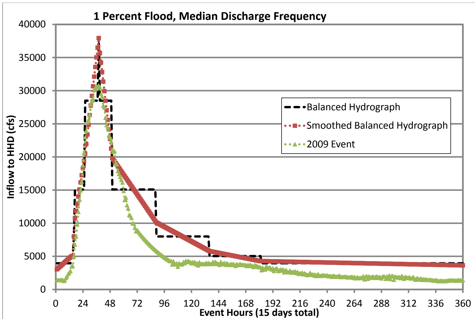
Figure 1 – Example balanced hydrograph, with shape and timing based on January 2009 flood event
