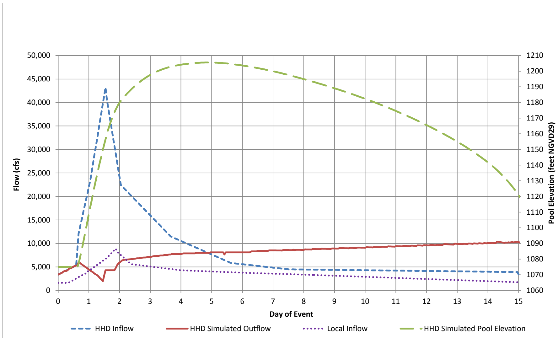
Figure 18 – Simulated Howard Hanson Dam Operations, 0.5 Percent Flood, Median Discharge Frequency Function
