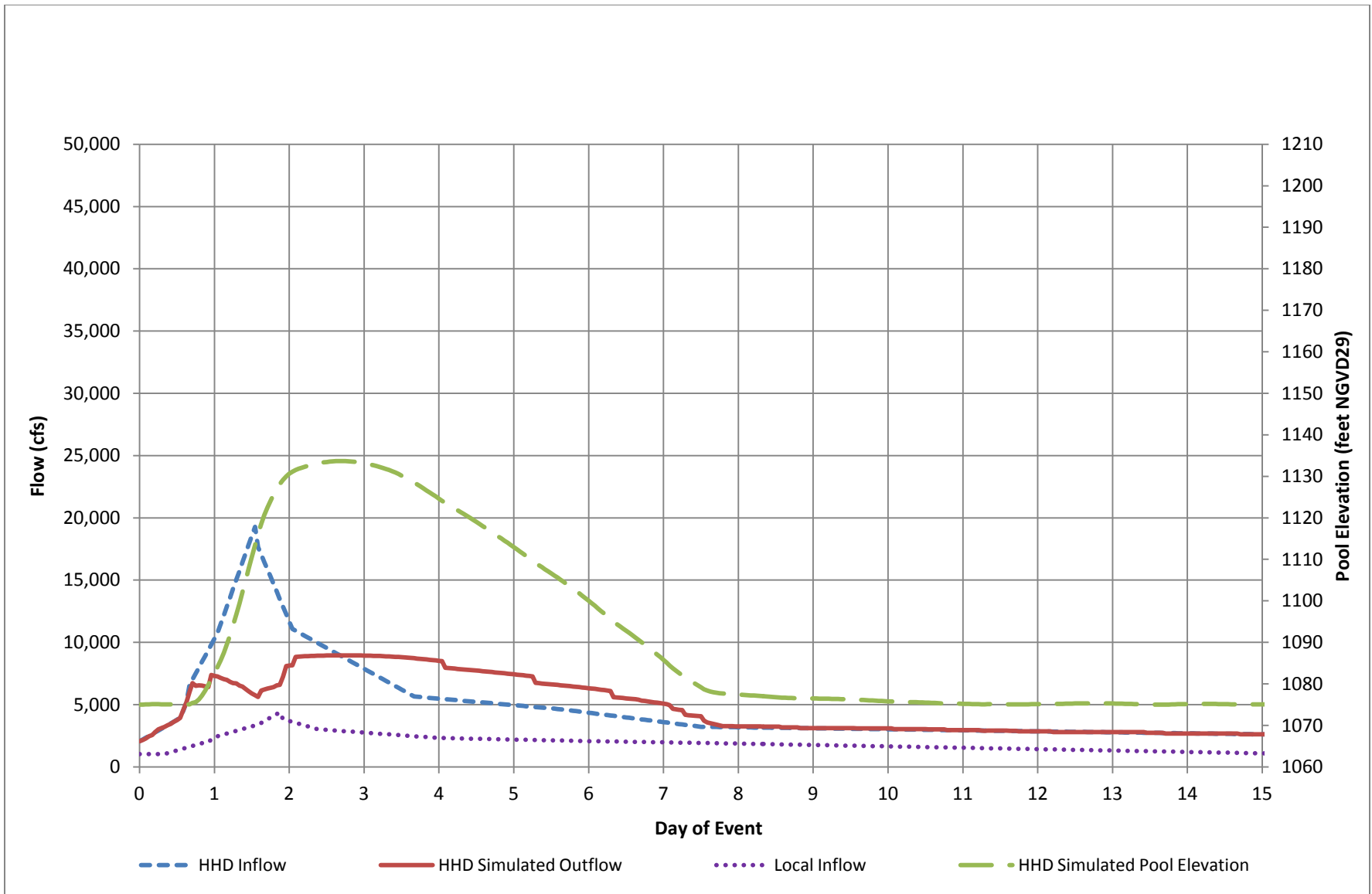
Figure 5 – Simulated Howard Hanson Dam Operations, 10 Percent Flood, Lower Confidence Limit (95%)
