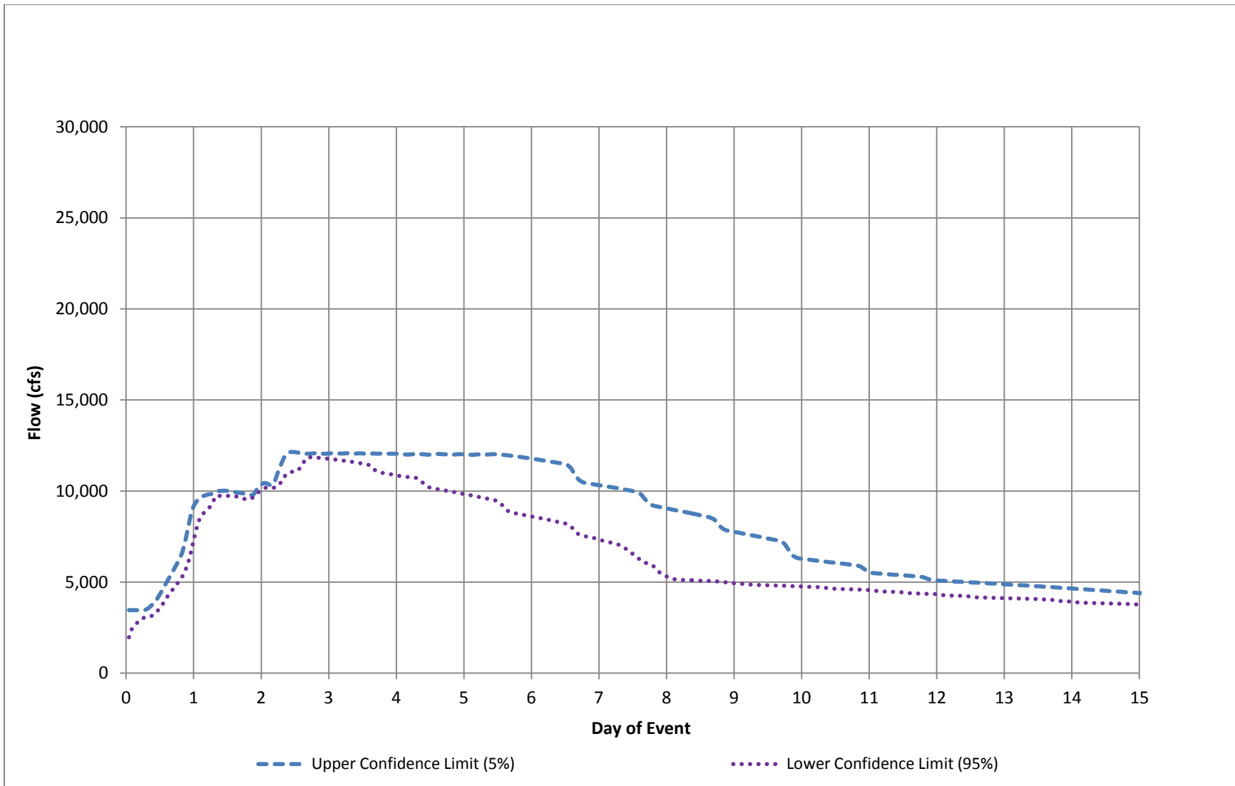
Figure 25 – Green River at Auburn Simulated Discharge, 10 Percent Flood
