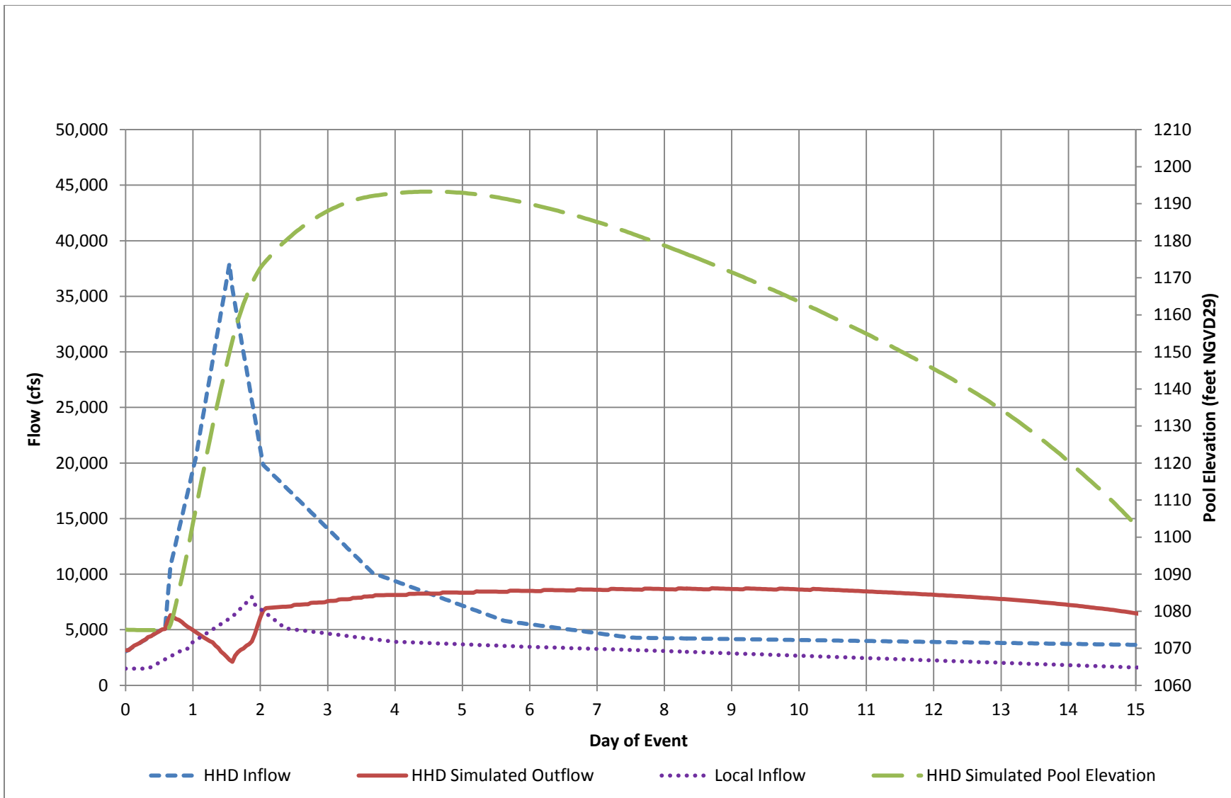
Figure 15 – Simulated Howard Hanson Dam Operations, 1 Percent Flood, Median Discharge Frequency Function
