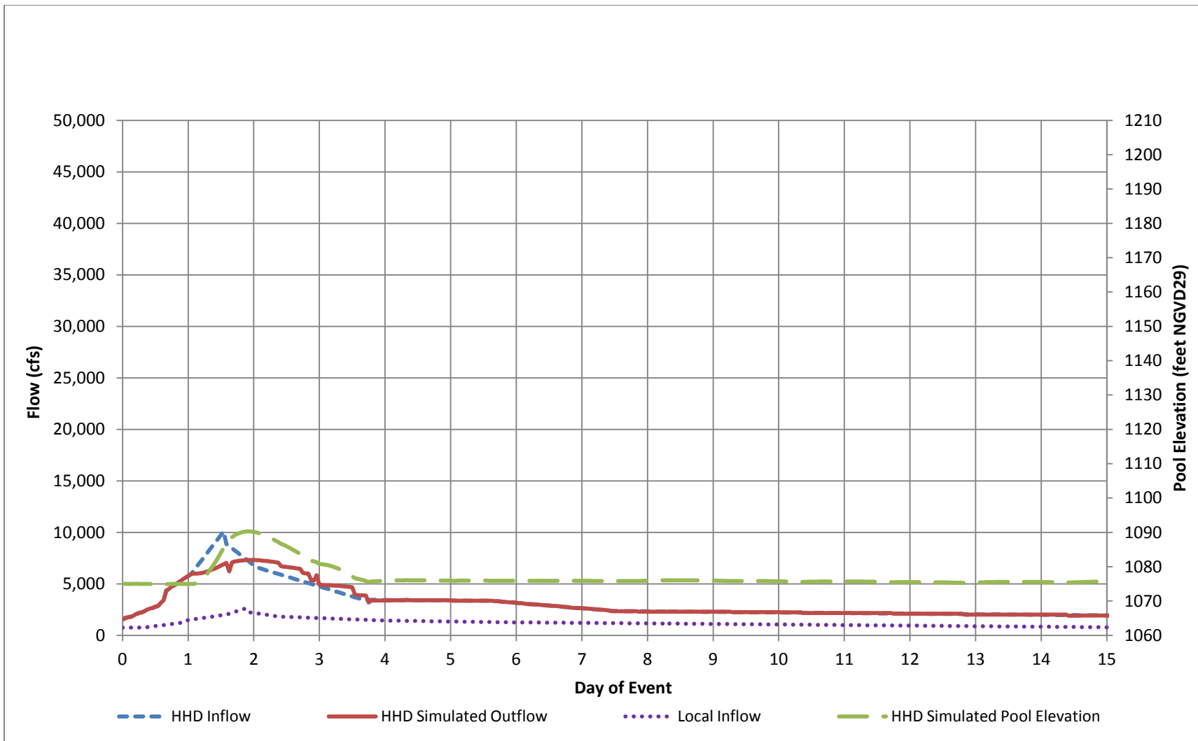
Figure 2 – Simulated Howard Hanson Dam Operations, 50 Percent Flood, Lower Confidence Limit (95%)
