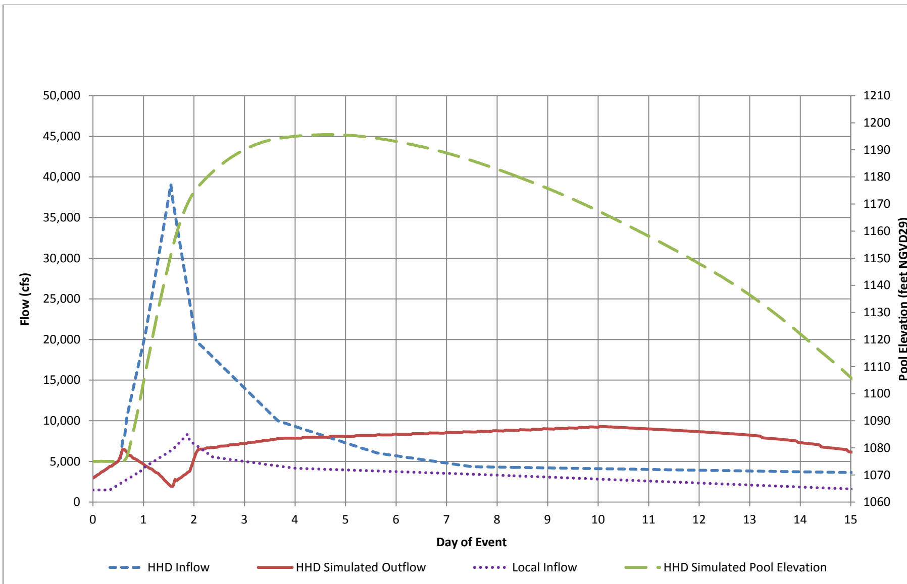
Figure 13 – Simulated Howard Hanson Dam Operations, 2 Percent Flood, Upper Confidence Limit (5%)
