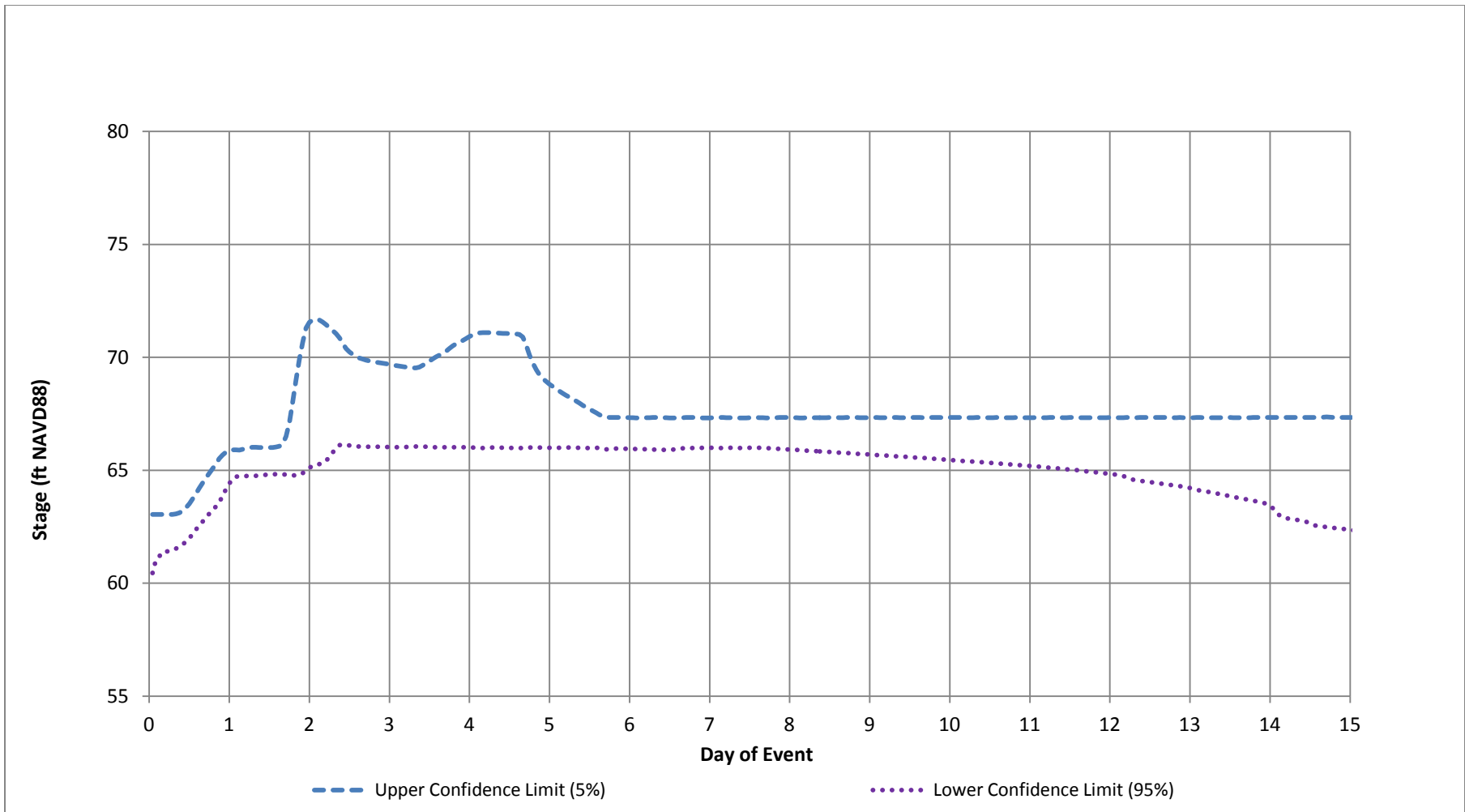
Figure 34 – Green River at Auburn Simulated Stage, 0.5 Percent Flood
