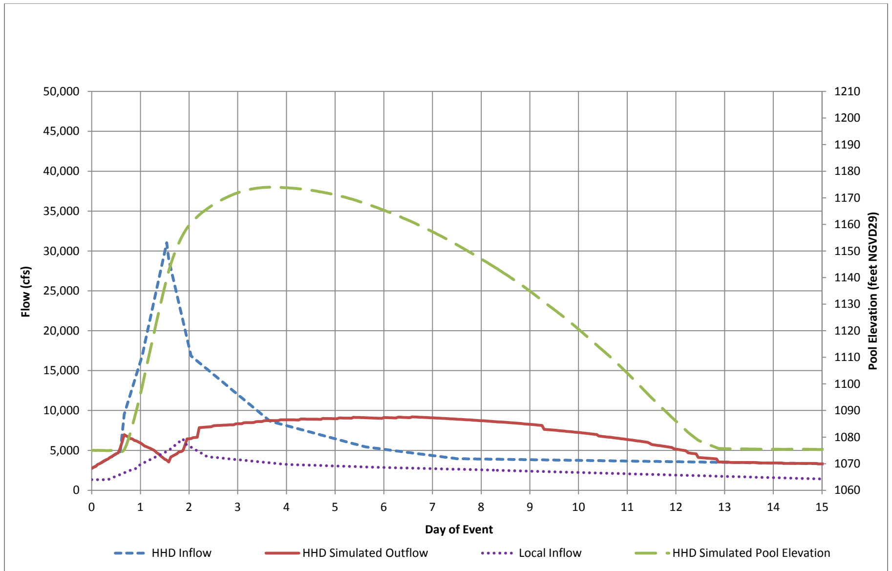
Figure 14 – Simulated Howard Hanson Dam Operations, 1 Percent Flood, Lower Confidence Limit (95%)
