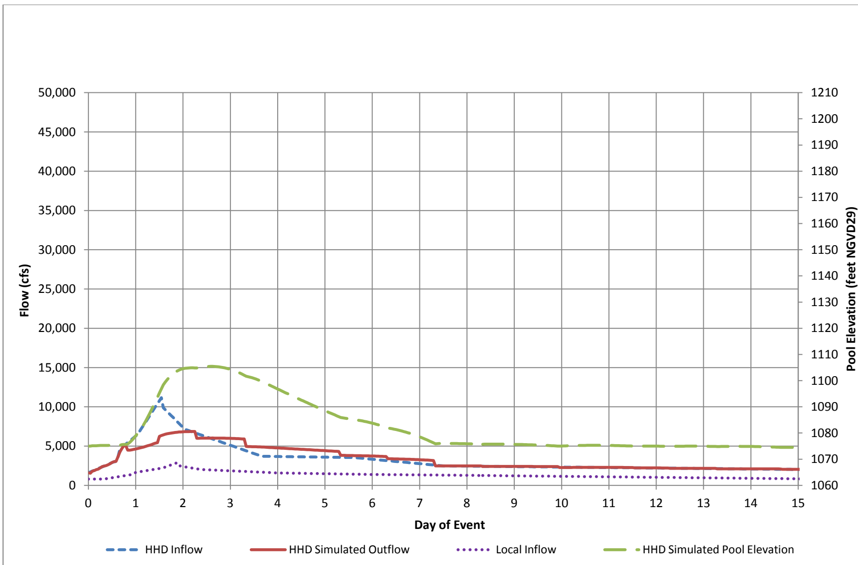
Figure 3 – Simulated Howard Hanson Dam Operations, 50 Percent Flood, Median Discharge Frequency Function
