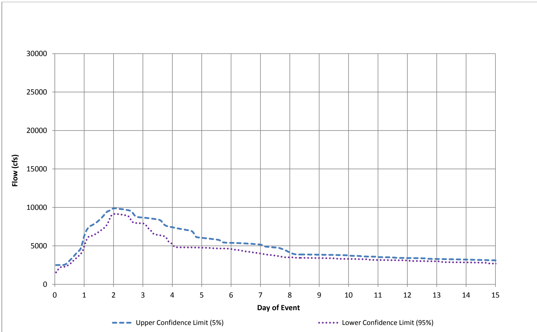
Figure 23 – Green River at Auburn Simulated Discharge, 50 Percent Flood
