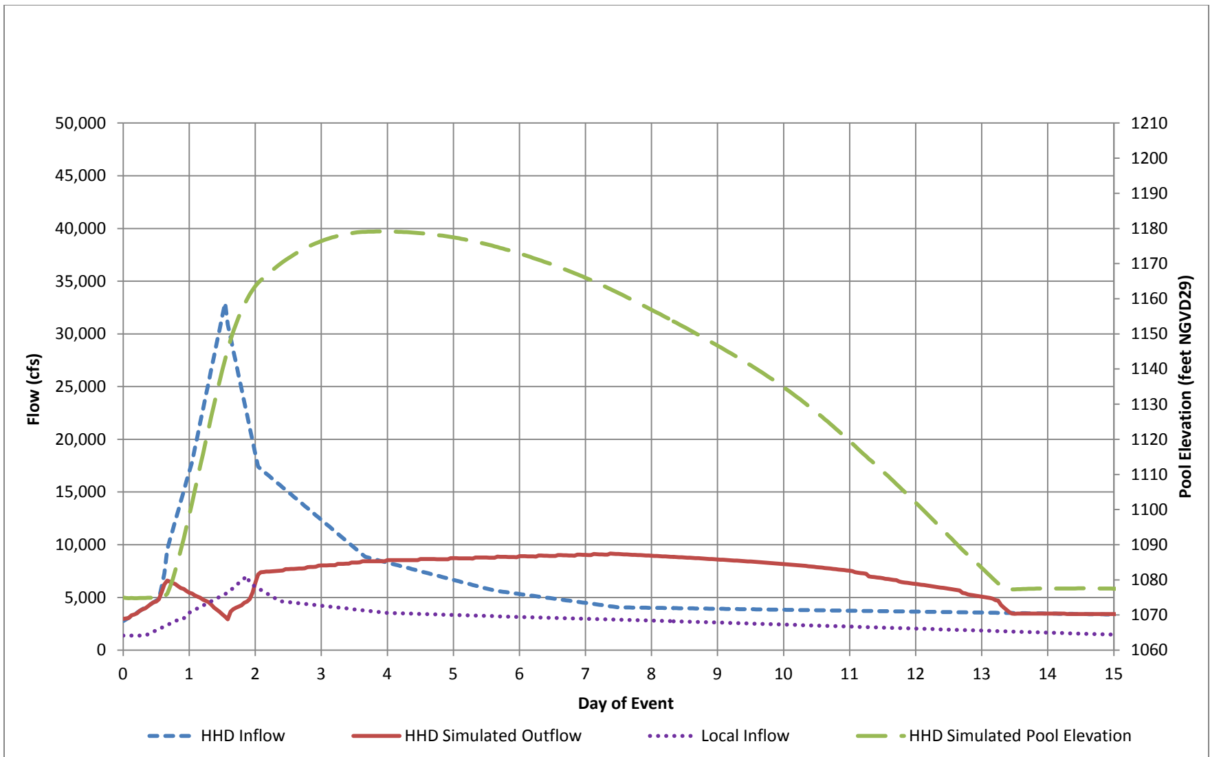
Figure 12 – Simulated Howard Hanson Dam Operations, 2 Percent Flood, Median Discharge Frequency Function
