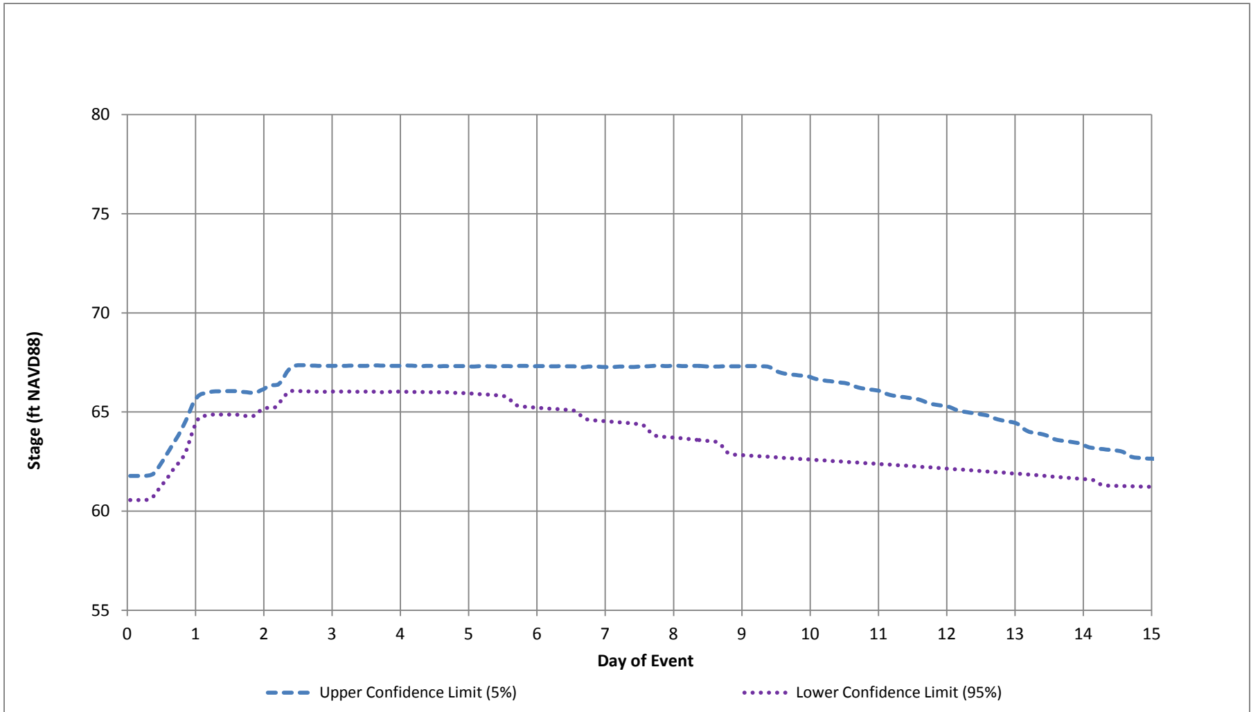
Figure 28 – Green River at Auburn Simulated Stage, 4 Percent Flood
