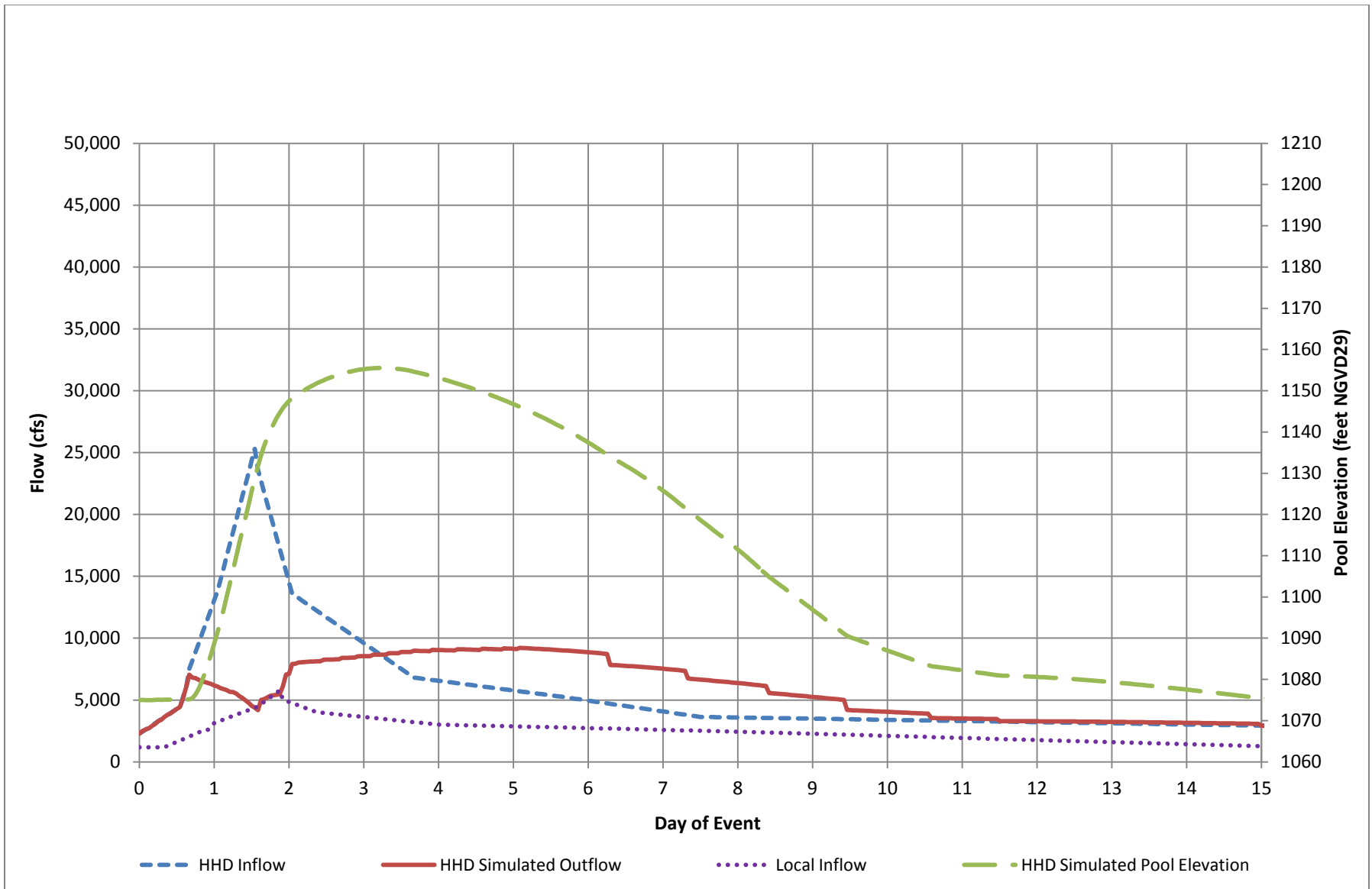
Figure 7 – Simulated Howard Hanson Dam Operations, 10 Percent Flood, Upper Confidence Limit (5%)
