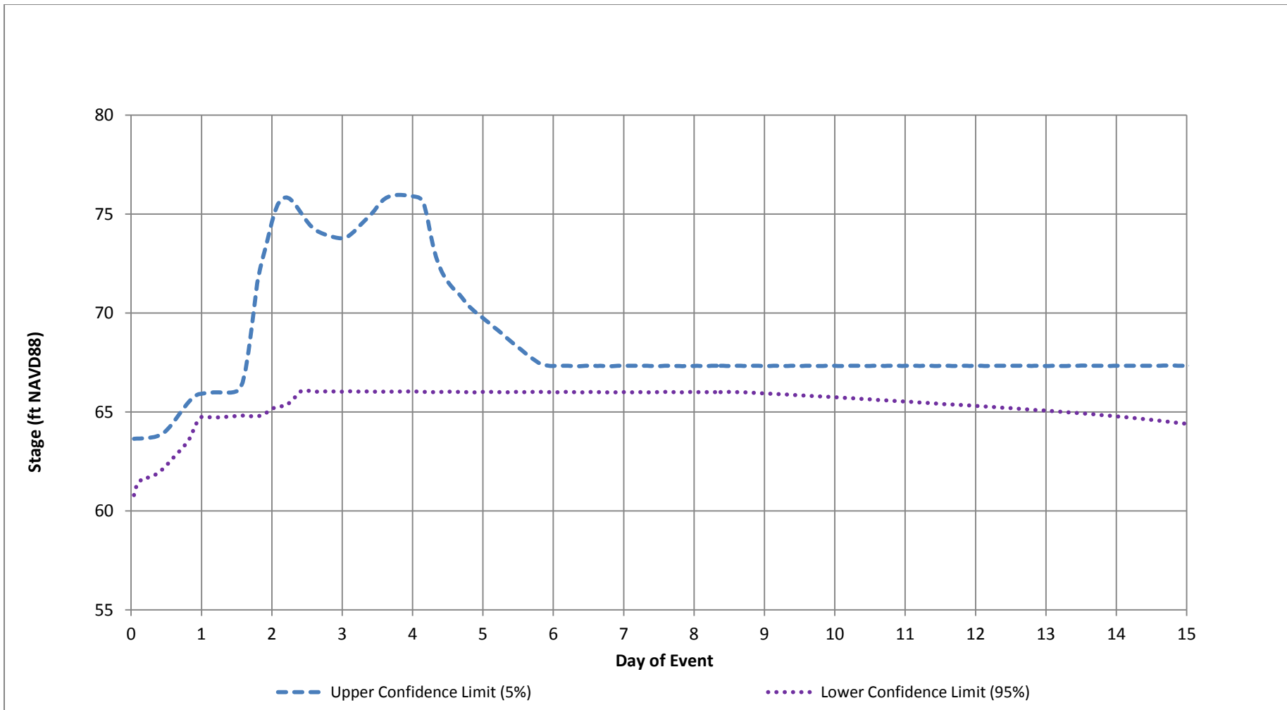
Figure 36 – Green River at Auburn Simulated Stage, 0.2 Percent Flood
