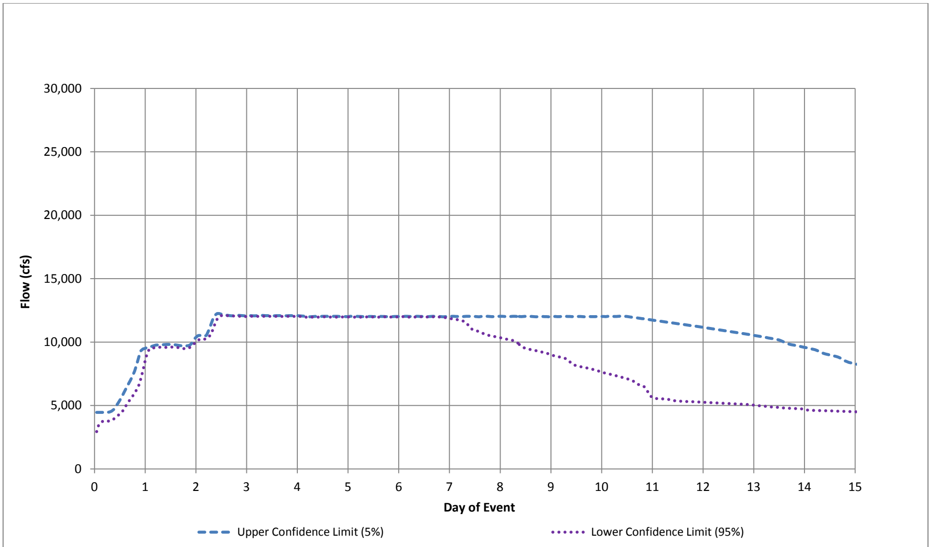
Figure 29 – Green River at Auburn Simulated Discharge, 2 Percent Flood
