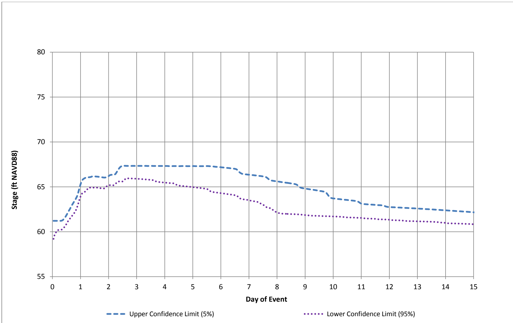
Figure 26 – Green River at Auburn Simulated Stage, 10 Percent Flood
