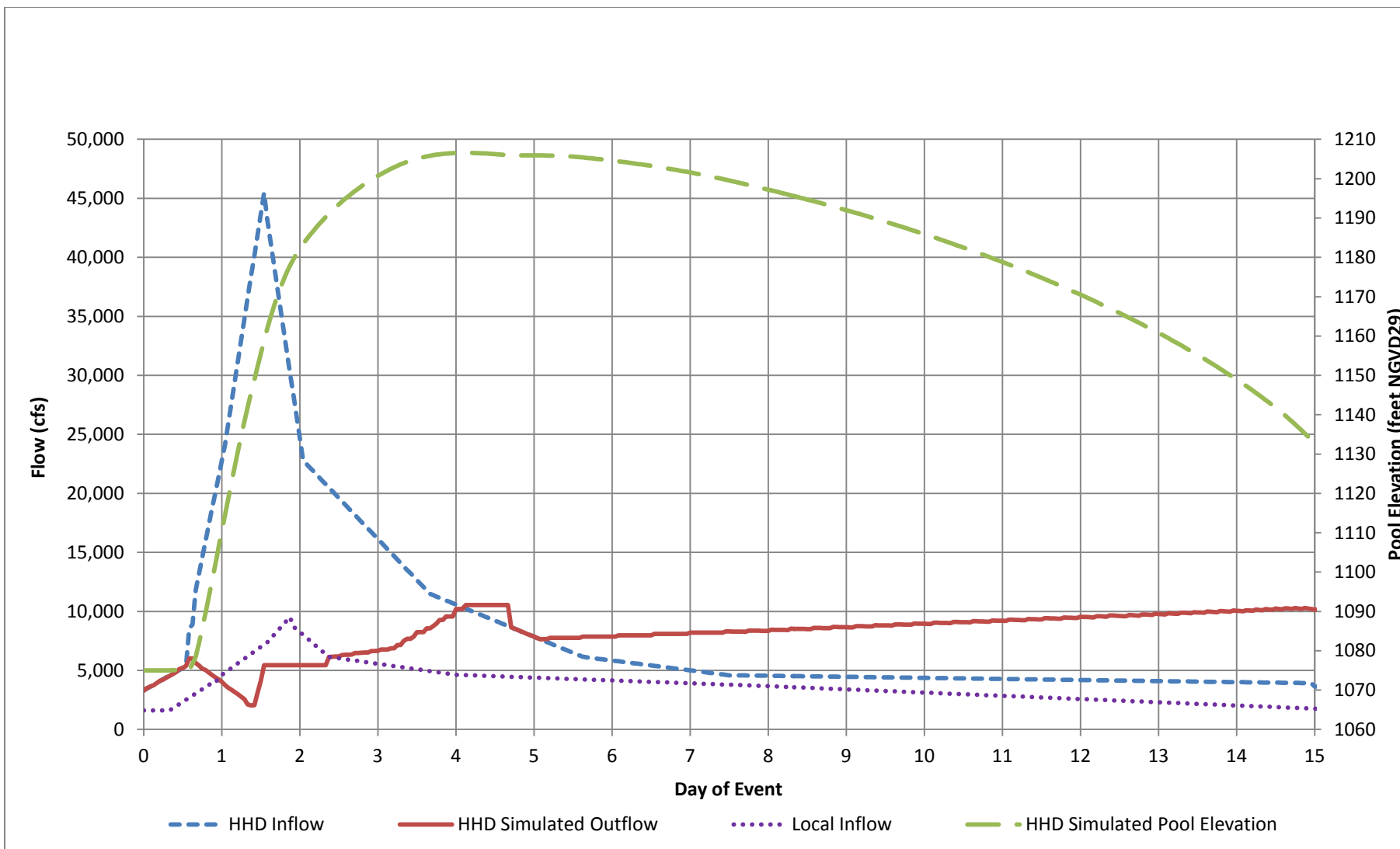
Figure 16 – Simulated Howard Hanson Dam Operations, 1 Percent Flood, Upper Confidence Limit (5%)
