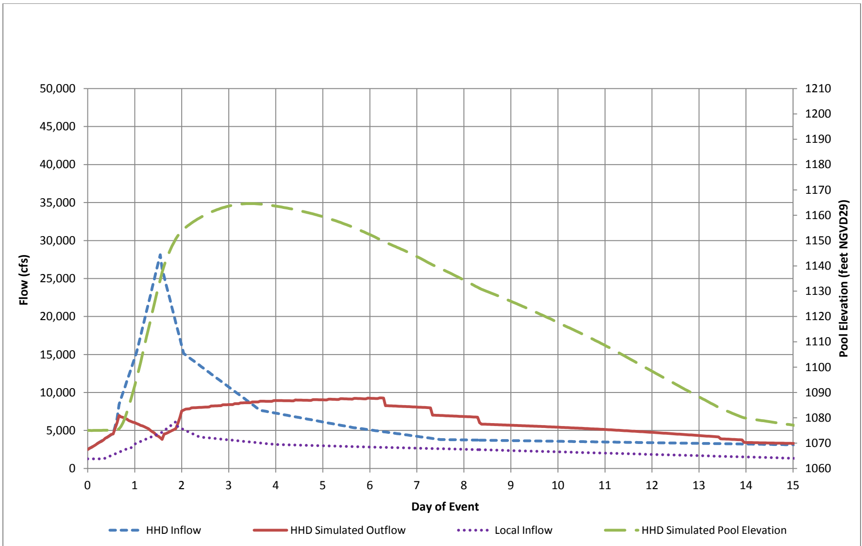
Figure 9 – Simulated Howard Hanson Dam Operations, 4 Percent Flood, Median Discharge Frequency Function
