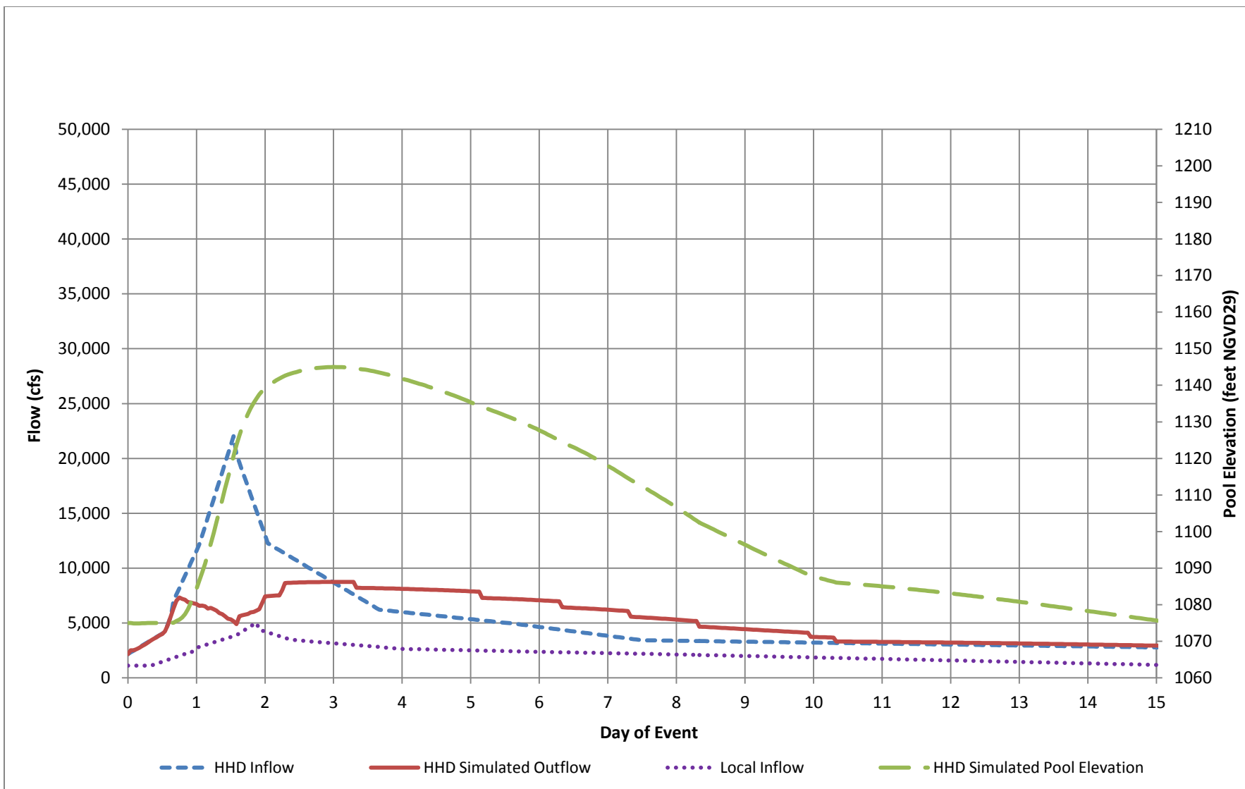
Figure 6 – Simulated Howard Hanson Dam Operations, 10 Percent Flood, Median Discharge Frequency Function
