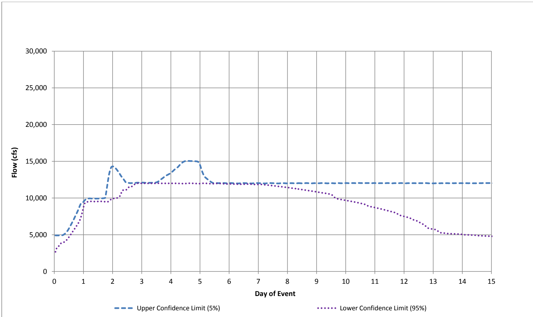
Figure 31 – Green River at Auburn Simulated Discharge, 1 Percent Flood
