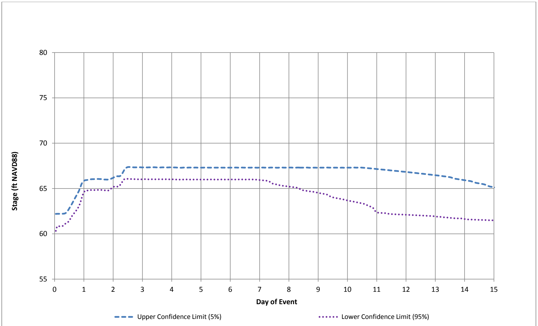
Figure 30 – Green River at Auburn Simulated Stage, 2 Percent Flood
