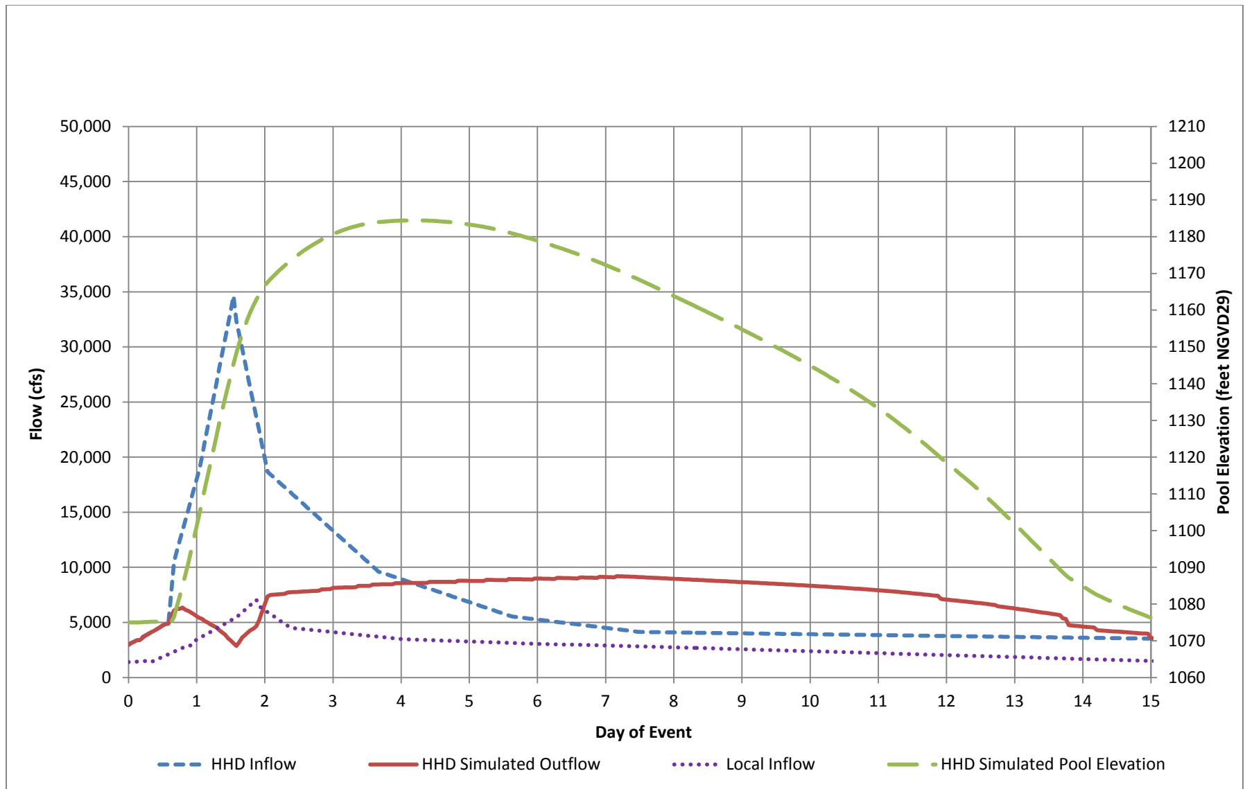
Figure 17 – Simulated Howard Hanson Dam Operations, 0.5 Percent Flood, Lower Confidence Limit (95%)
