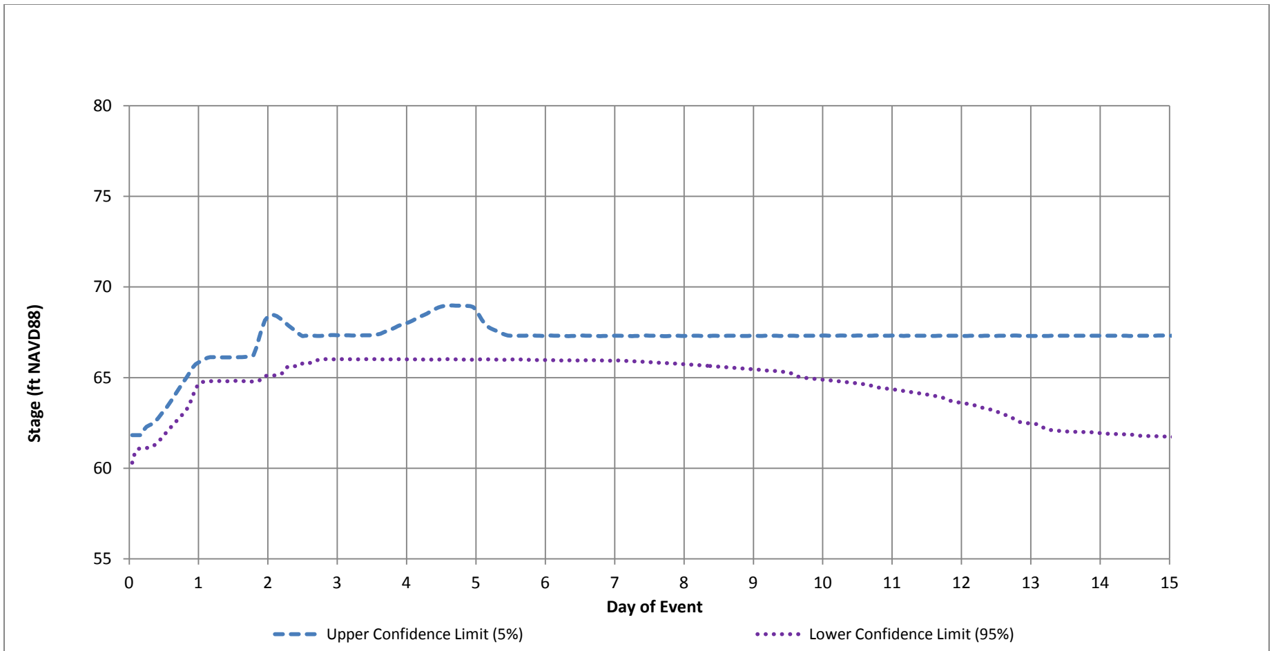
Figure 32 – Green River at Auburn Simulated Stage, 1 Percent Flood
