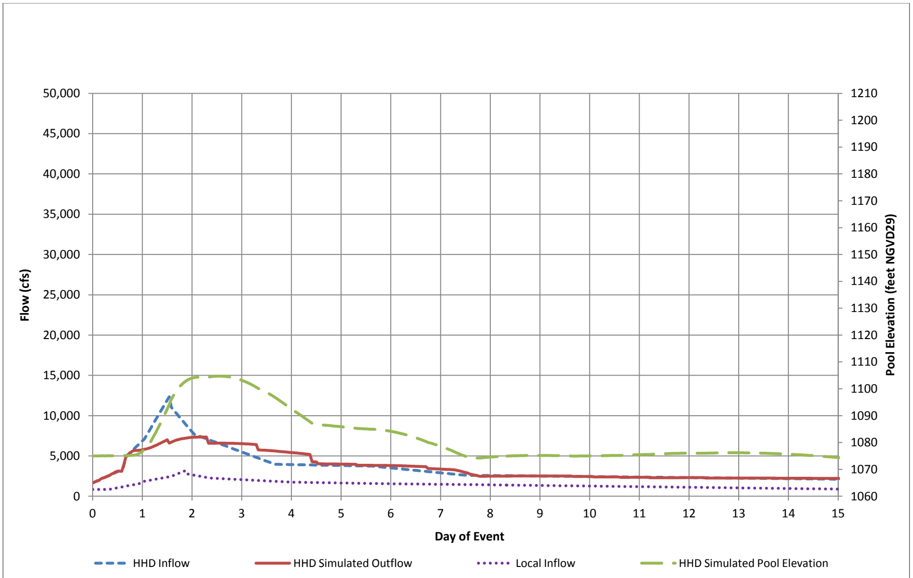
Figure 4 – Simulated Howard Hanson Dam Operations, 50 Percent Flood, Upper Confidence Limit (5%)
