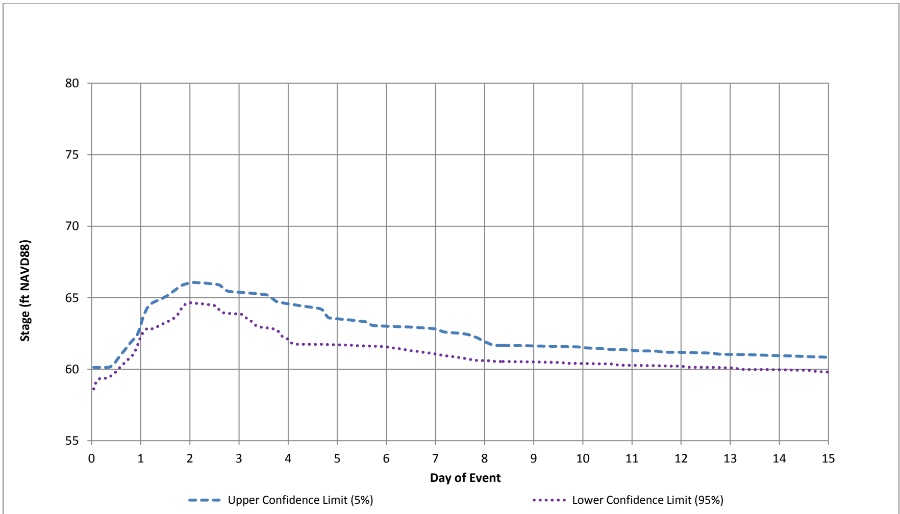
Figure 24 – Green River at Auburn Simulated Stage, 50 Percent Flood
