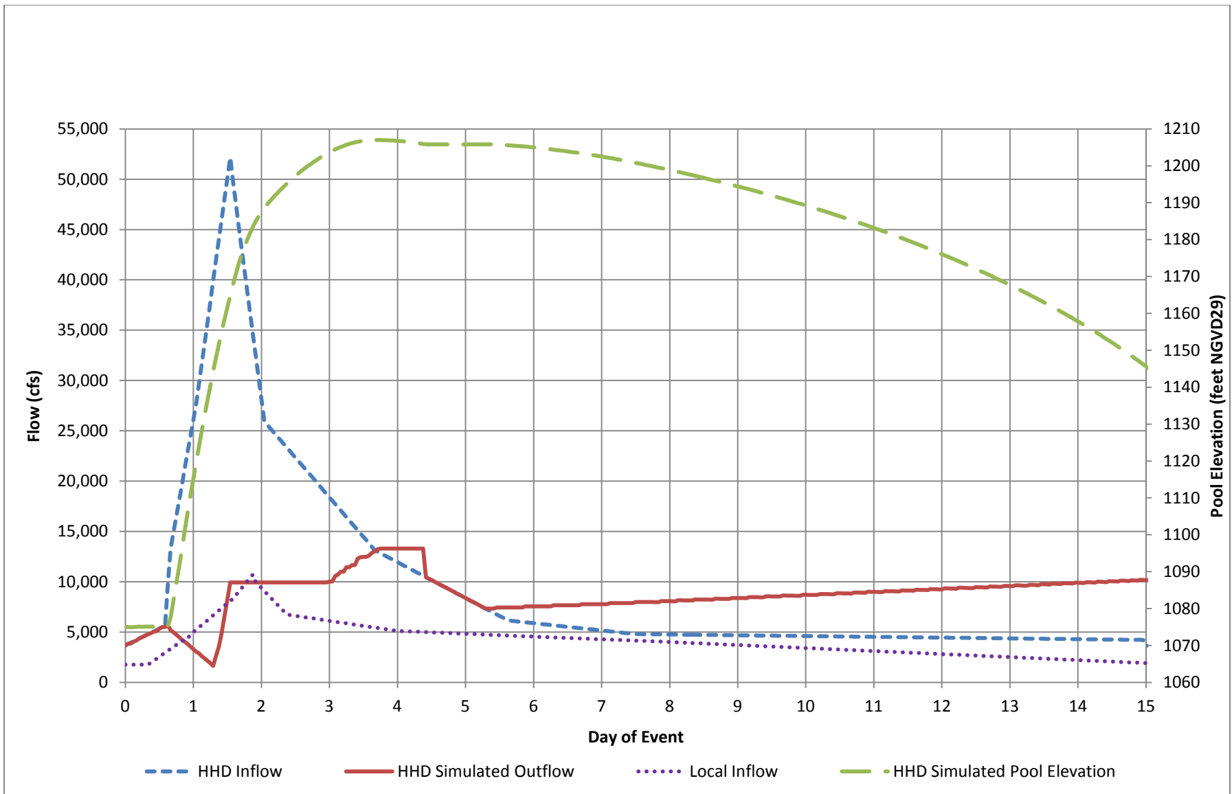
Figure 19 – Simulated Howard Hanson Dam Operations, 0.5 Percent Flood, Upper Confidence Limit (5%)
