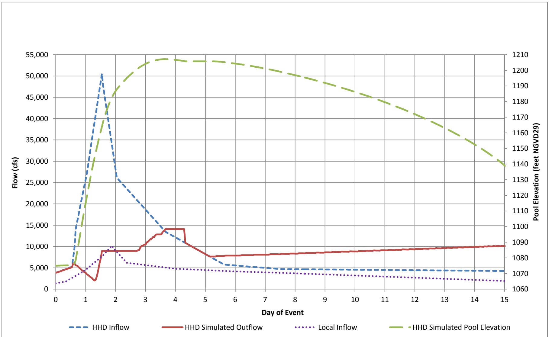
Figure 21 – Simulated Howard Hanson Dam Operations, 0.2 Percent Flood, Median Discharge Frequency Function
