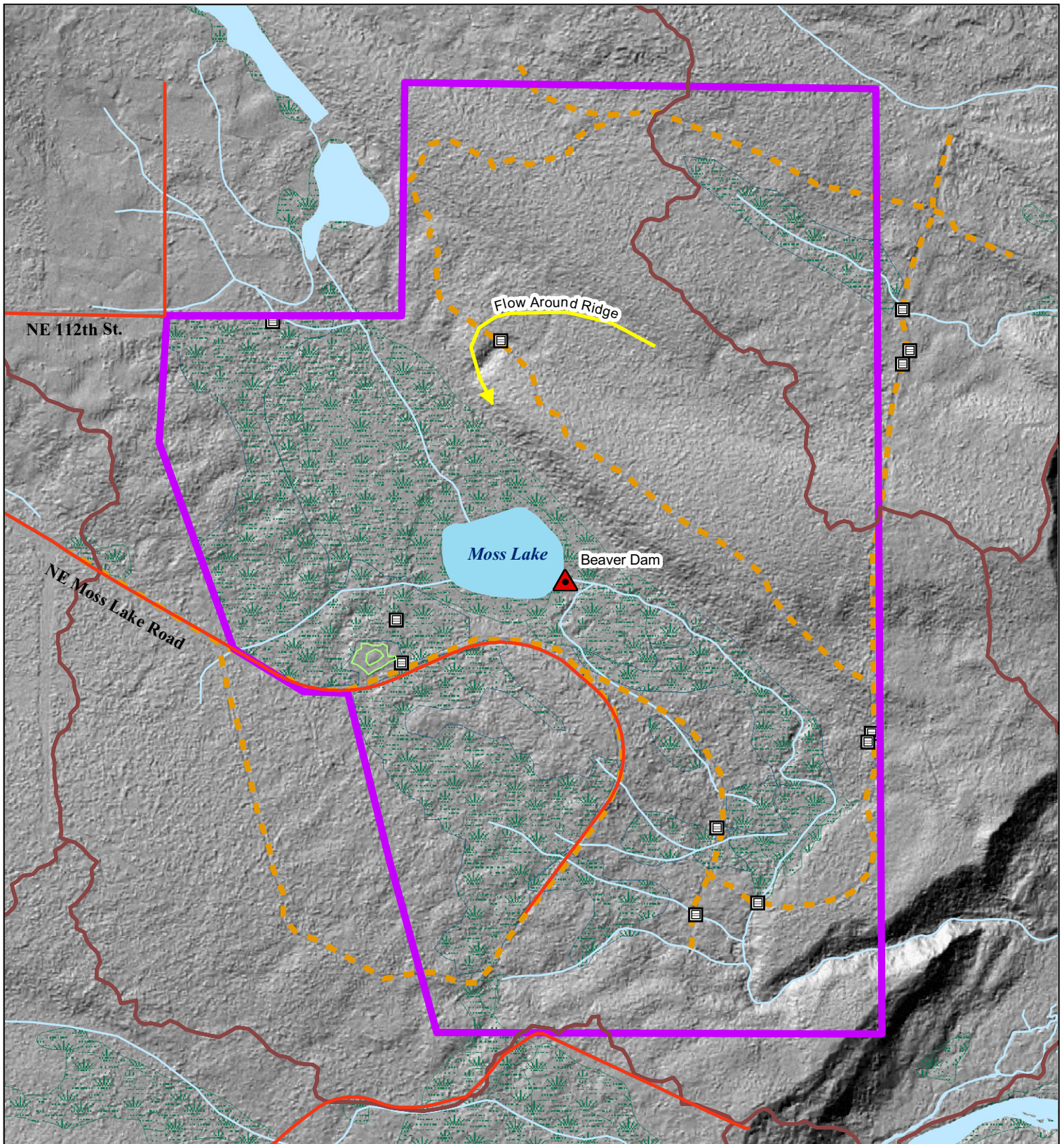
Figure 6: Hydrology Map
