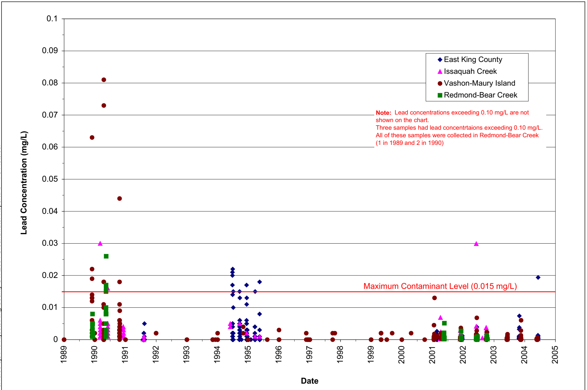
Figure 12 Lead in Four Groundwater Management Areas King County Ambient Groundwater Monitoring Program
