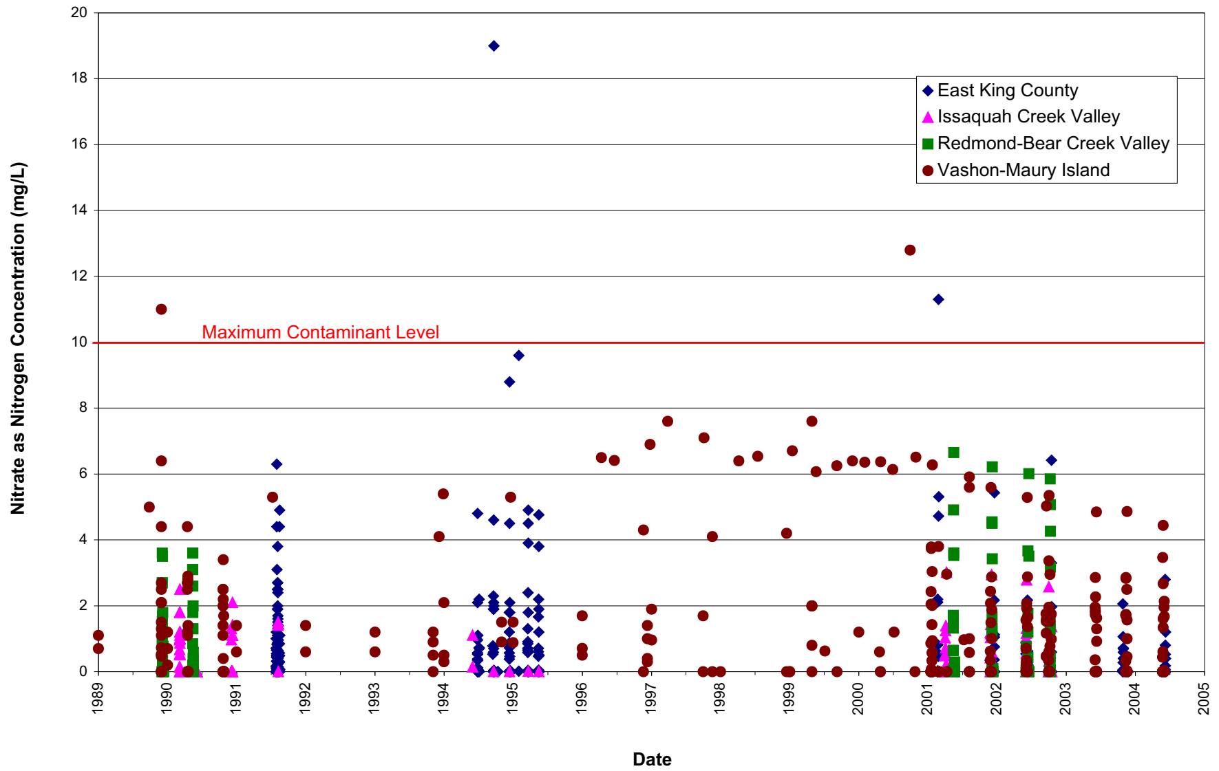
Figure 11 Nitrate in Four Groundwater Management Areas King County Ambient Groundwater Monitoring Program
