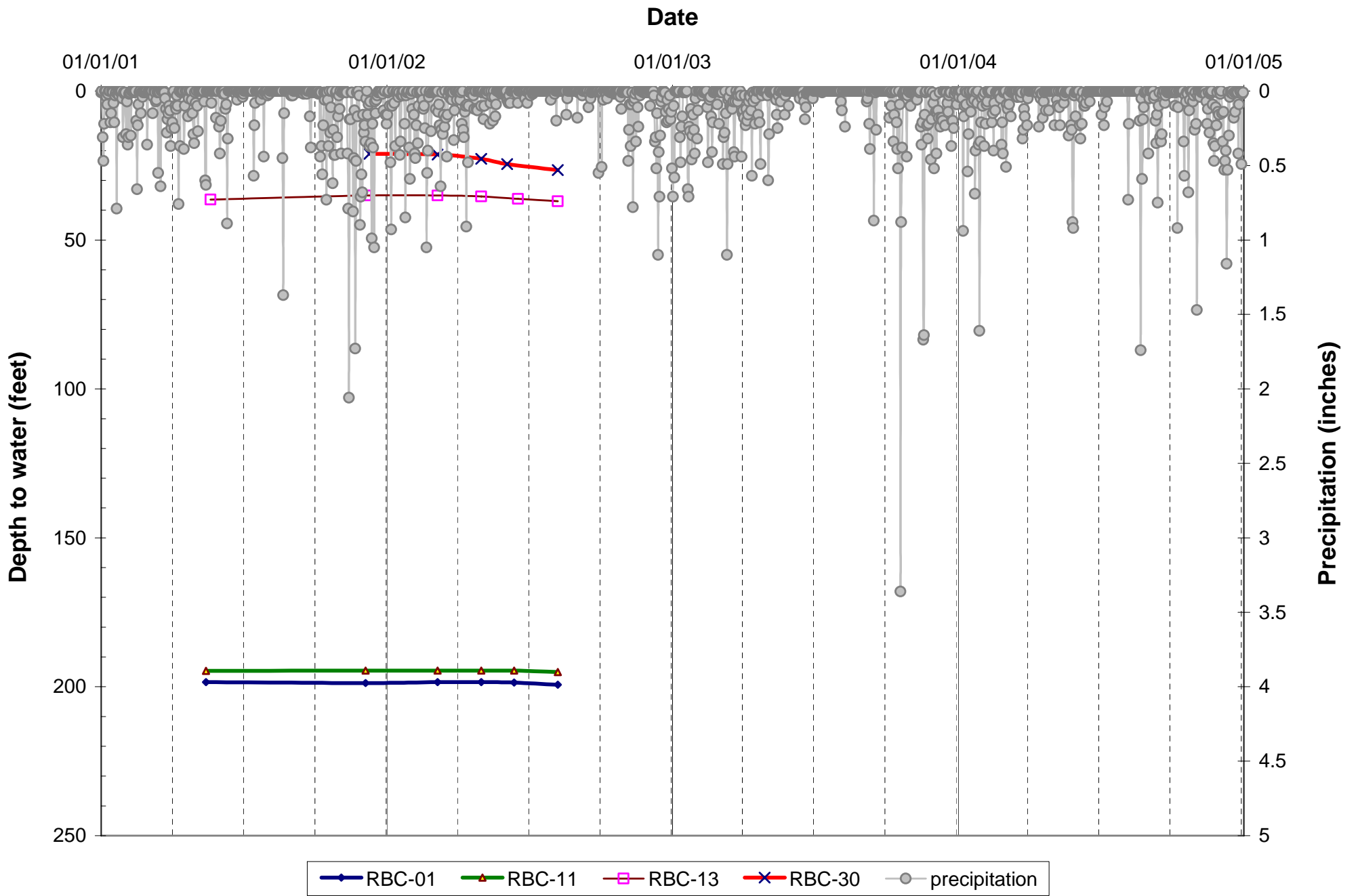
Figure 8C Hydrographs: Redmond-Bear Creek GWMA King County Ambient Groundwater Monitoring Program
