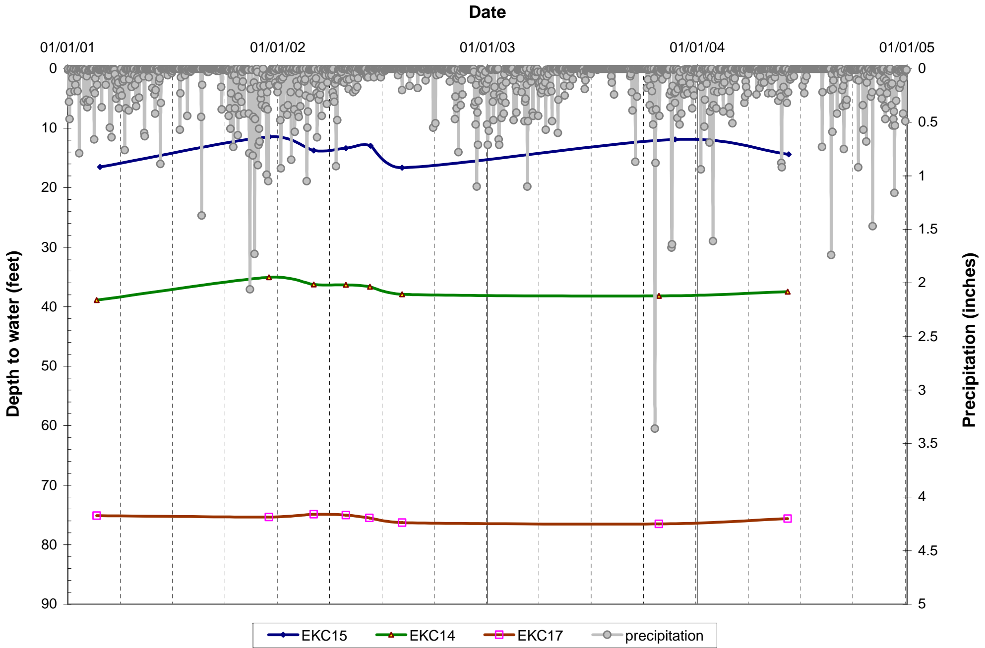
Figure 8A Hydrographs: East King County GWMA King County Ambient Groundwater Monitoring Program
