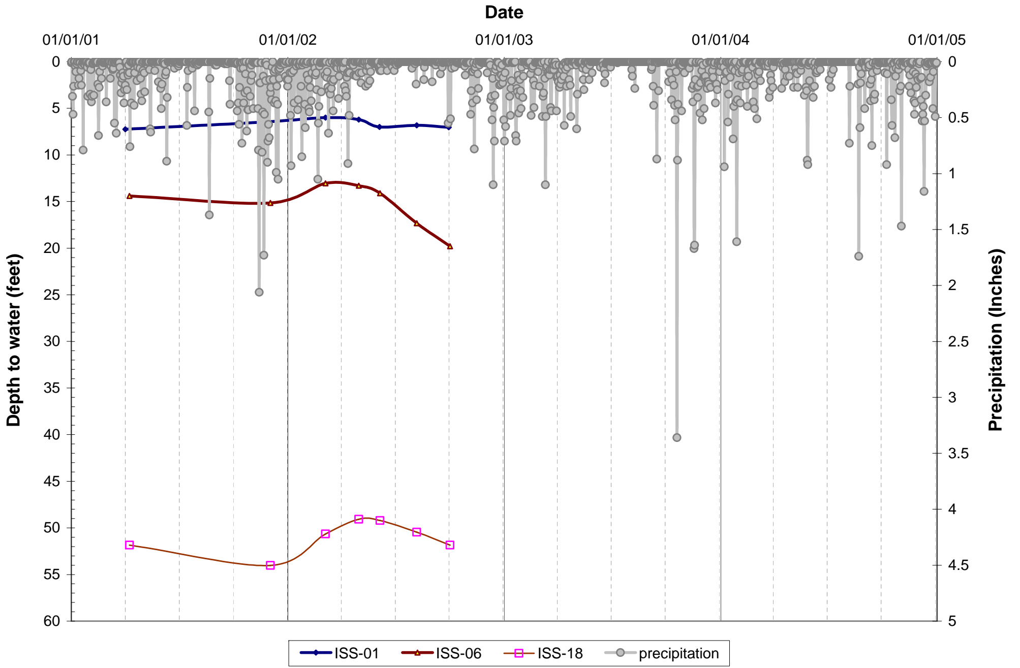
Figure 8B Hydrographs: Issaquah Creek Valley GWMA King County Ambient Groundwater Monitoring Program
