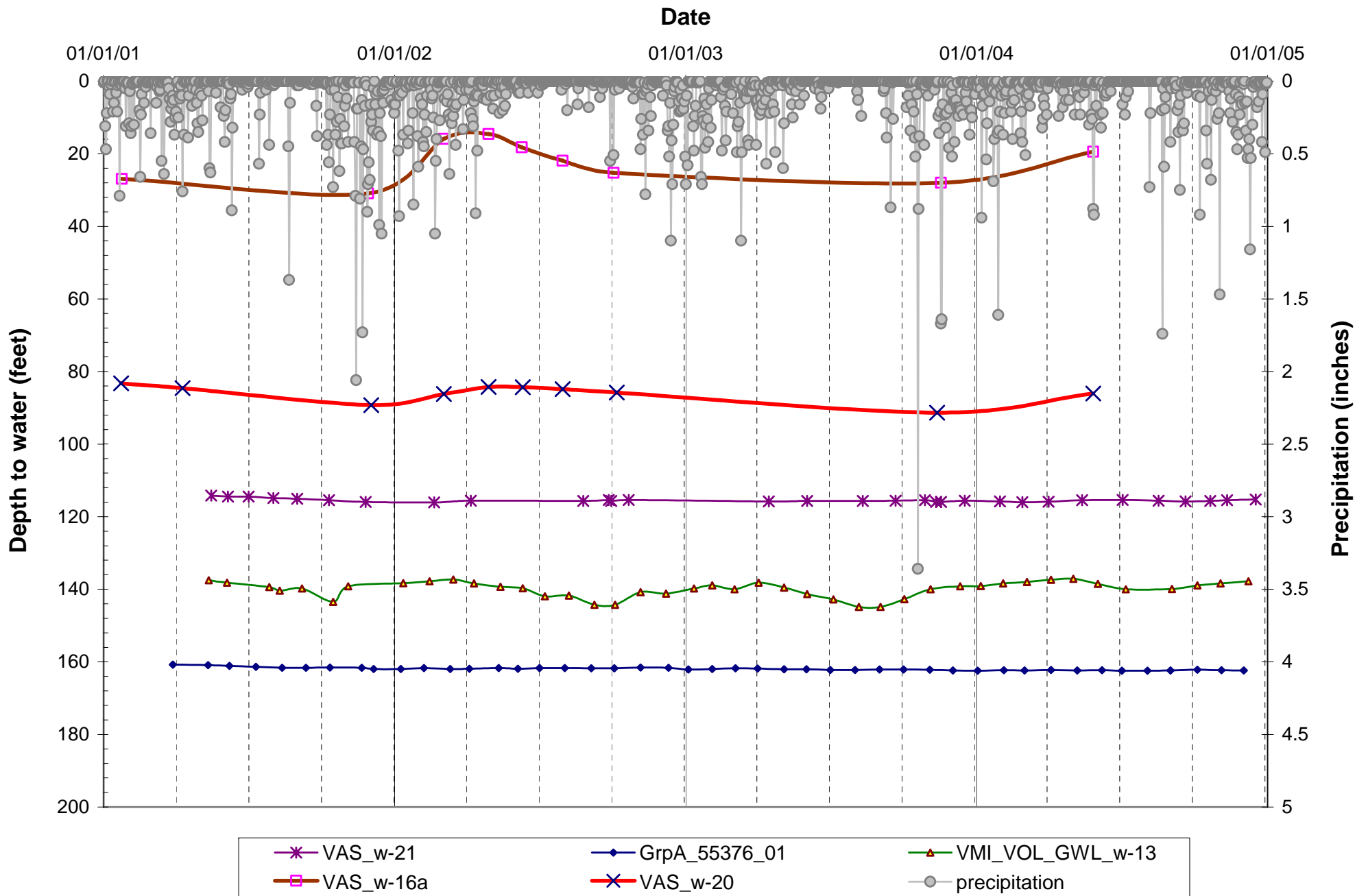
Figure 8D Hydrographs: Vashon-Maury Island GWMA King County Ambient Groundwater Monitoring Program
