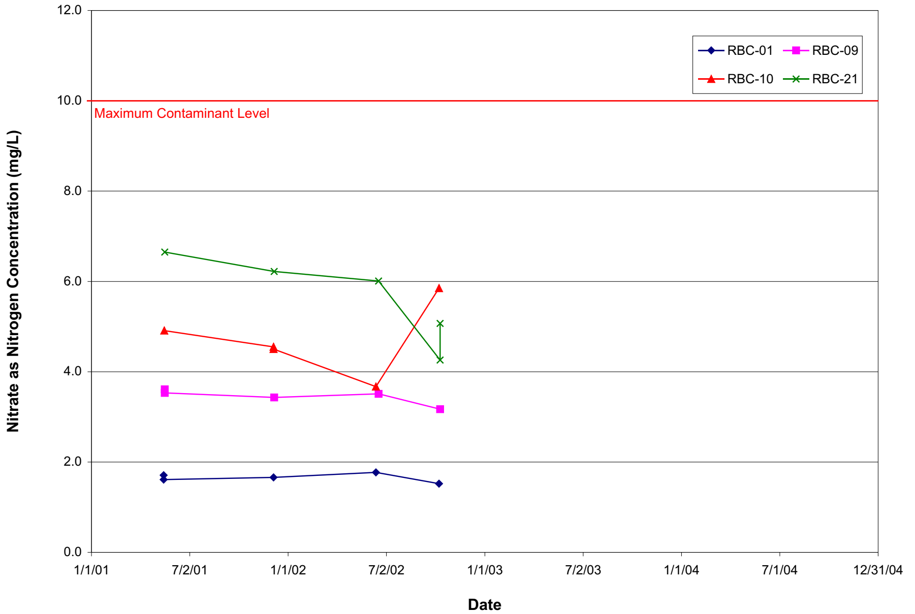
Figure 6C Nitrate Concentrations in Selected Wells: Redmond-Bear Creek Valley GWMA King County Ambient Groundwater Monitoring Program
