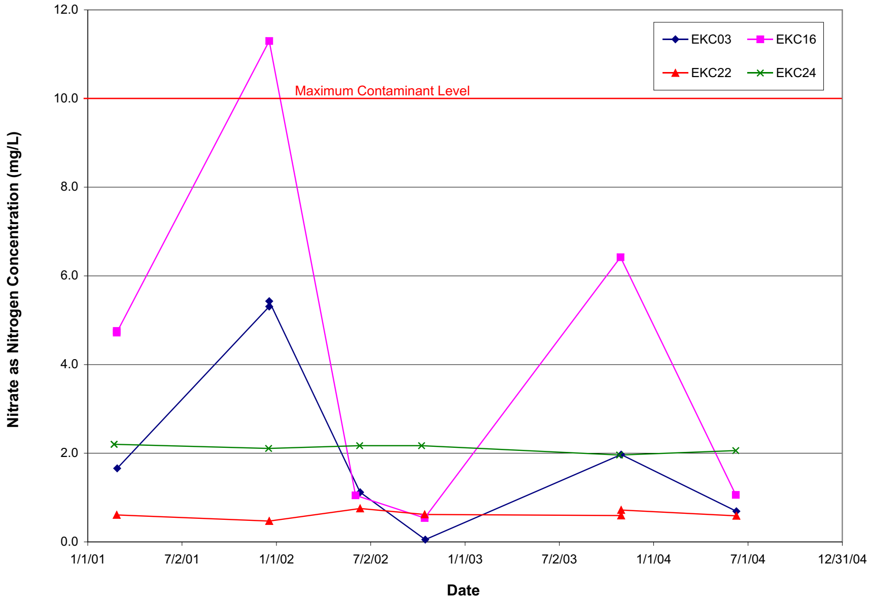
Figure 6A Nitrate Concentrations in Selected Wells: East King County GWMA King County Ambient Groundwater Monitoring Program
