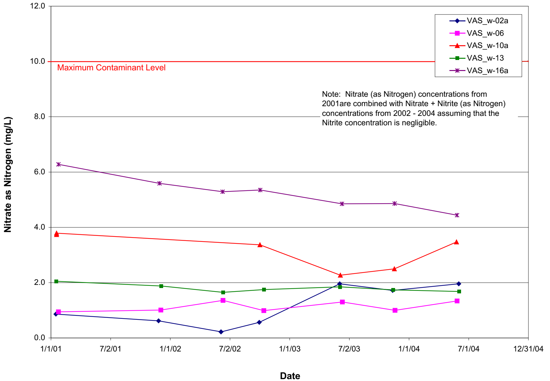
Figure 6D Nitrate Concentrations in Selected Wells: Vashon-Maury Island GWMA King County Ambient Groundwater Monitoring Program
