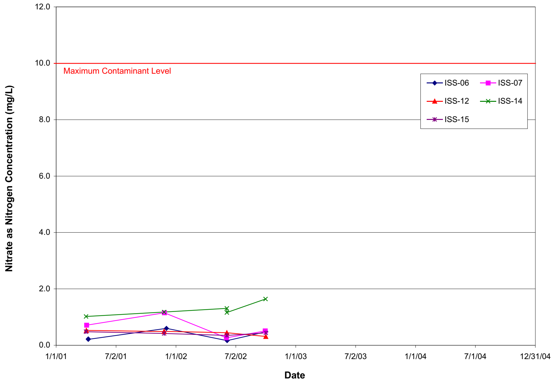
Figure 6B Nitrate Concentrations in Selected Wells: Issaquah Creek Valley GWMA King County Ambient Groundwater Monitoring Program
