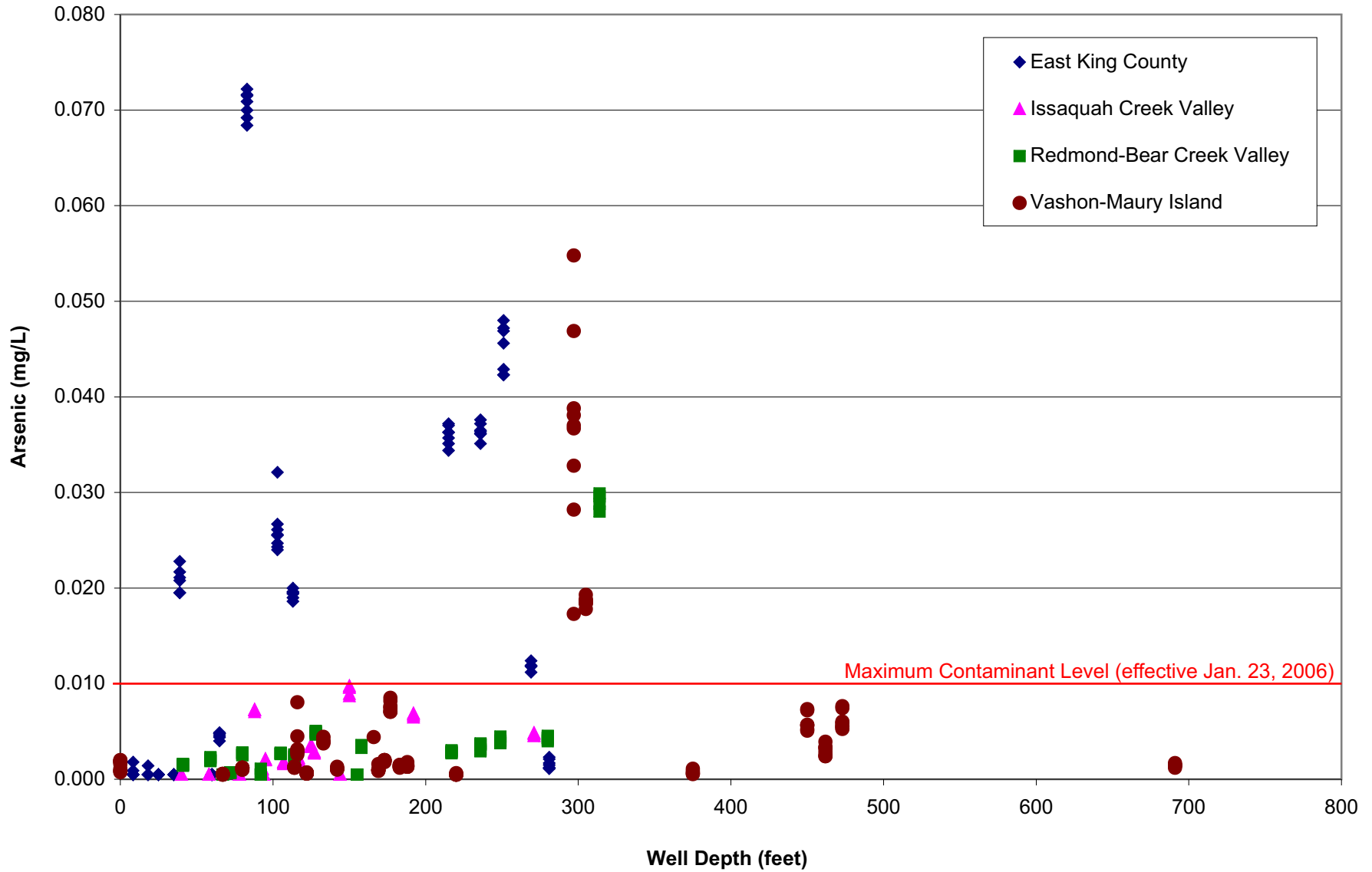
Figure 5 Arsenic Concentrations versus Well Depth: All Groundwater Management Areas (2001 - 2004) King County Ambient Groundwater Monitoring Program
