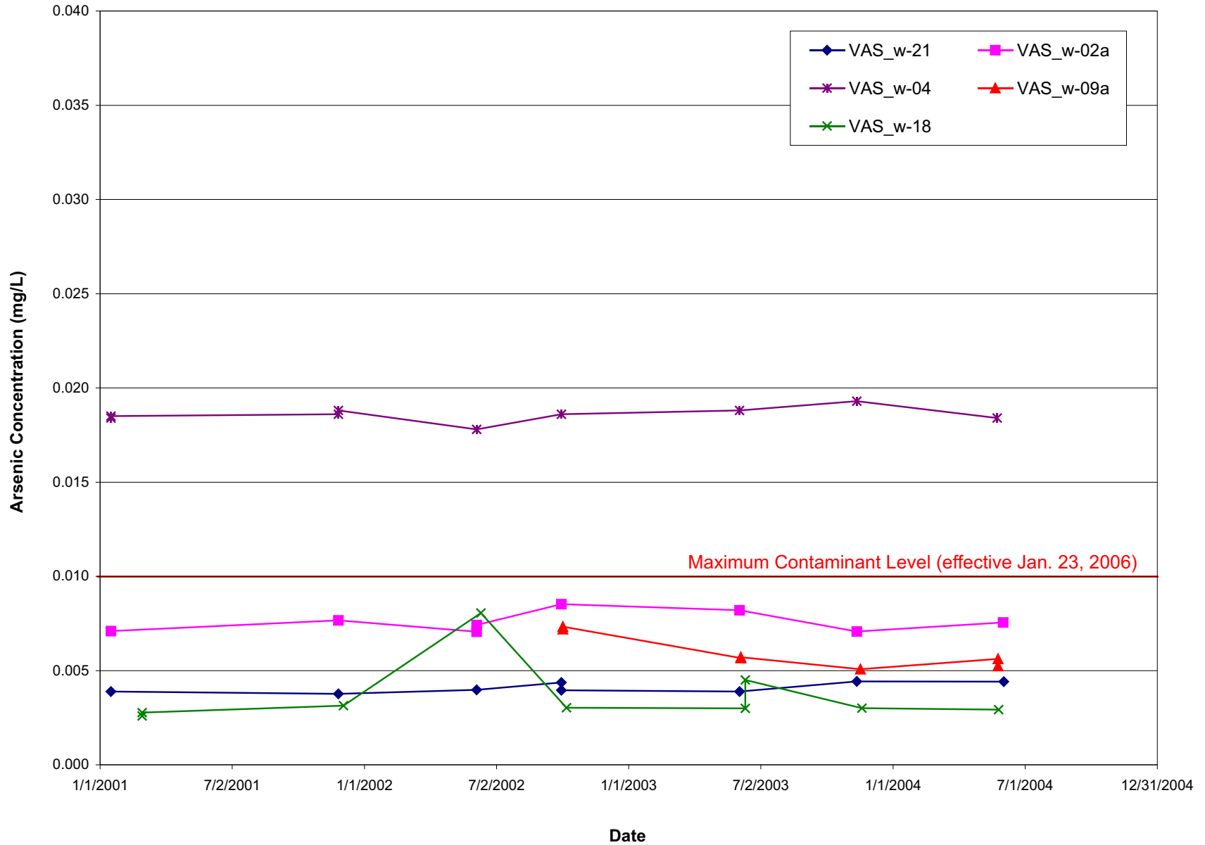
Figure 4D Arsenic Concentrations in Selected Wells: Vashon-Maury Island GWMA King County Ambient Groundwater Monitoring Program
