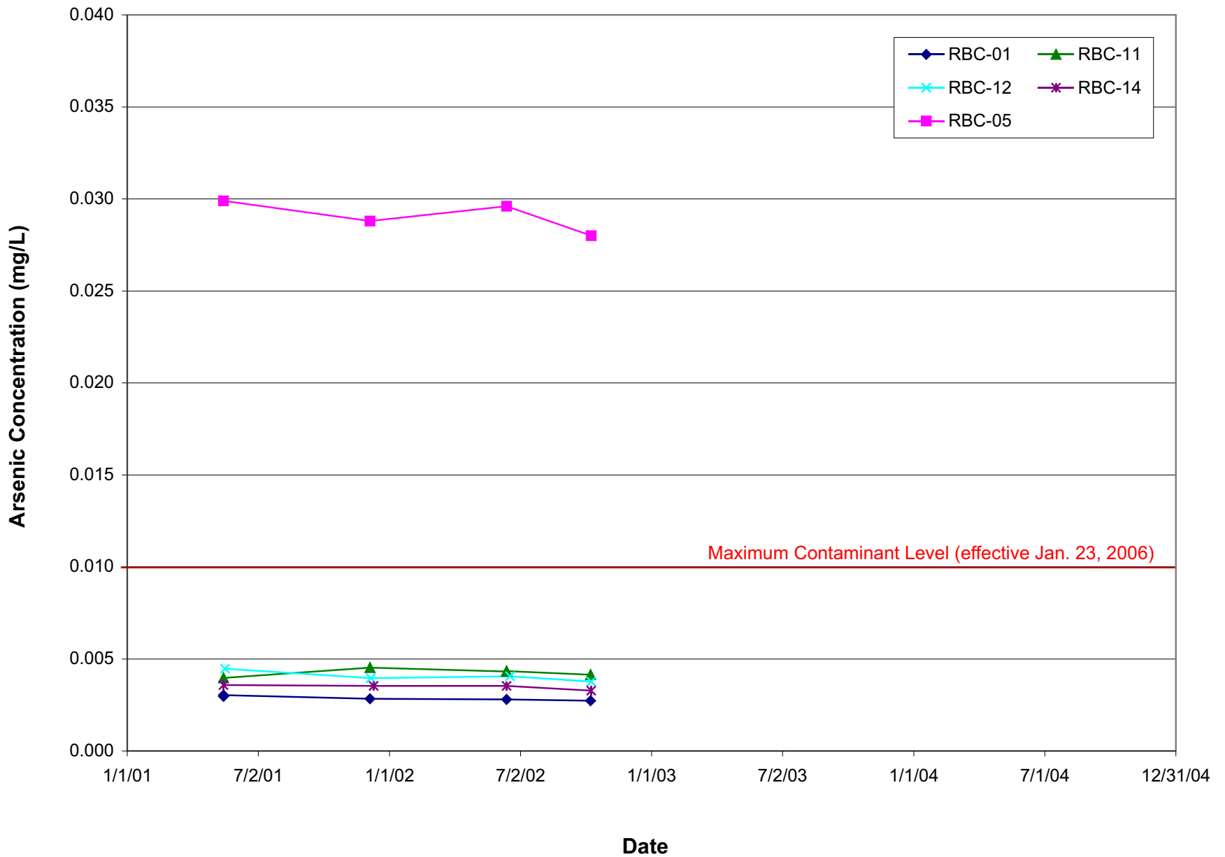
Figure 4C Arsenic Concentrations in Selected Wells: Redmond-Bear Creek Valley GWMA King County Ambient Groundwater Monitoring Program
