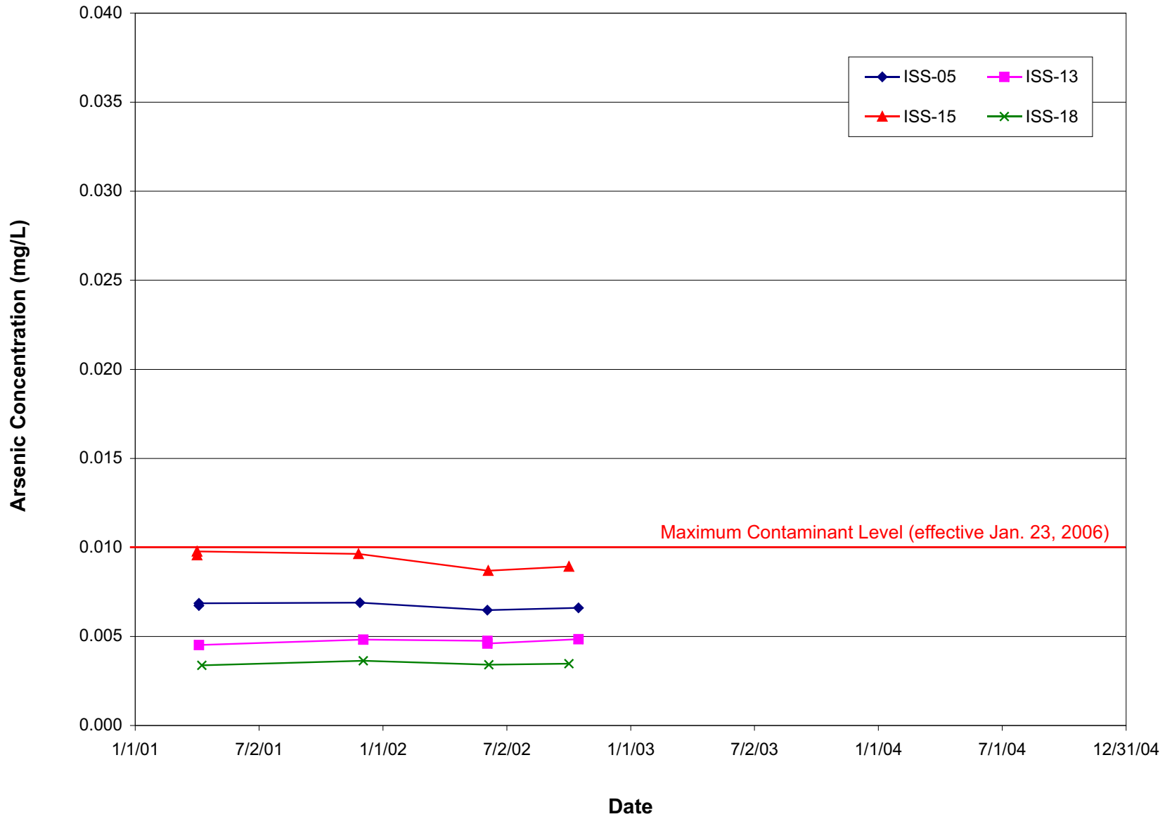
Figure 4B Arsenic Concentrations in Selected Wells: Issaquah Creek Valley GWMA King County Ambient Groundwater Monitoring Program
