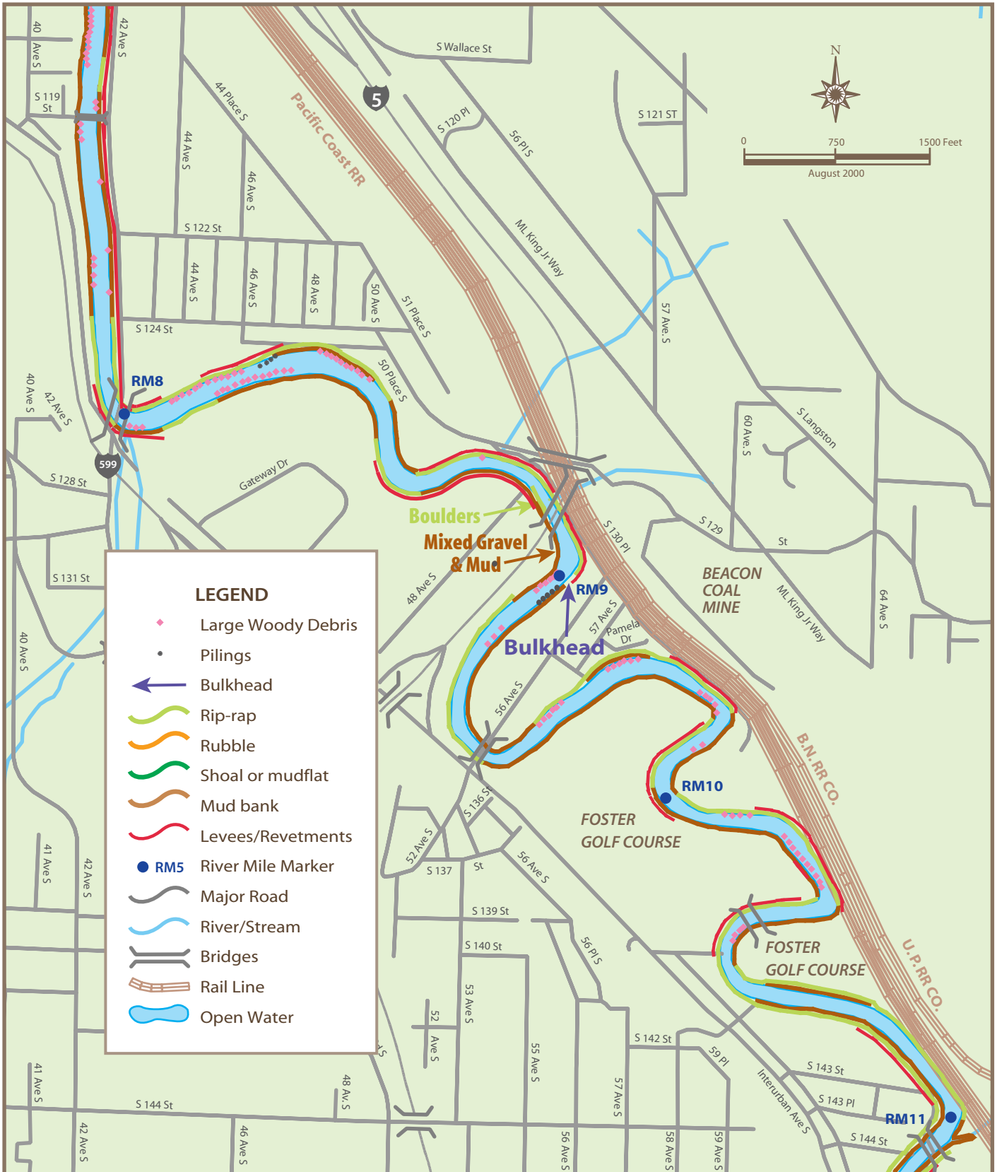
Figure 24 Artificial Channel Constraints and Large Woody Debris
