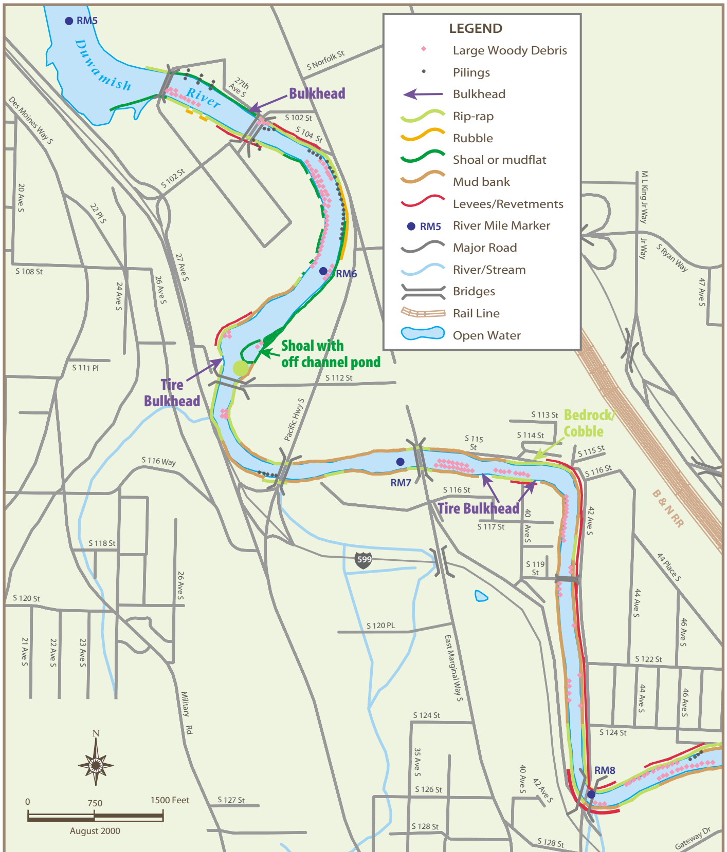
Figure HM-8-1 Artificial Channel Constraints and Large Woody Debris Green-Duwamish River Estuary - Map 1 of 3
