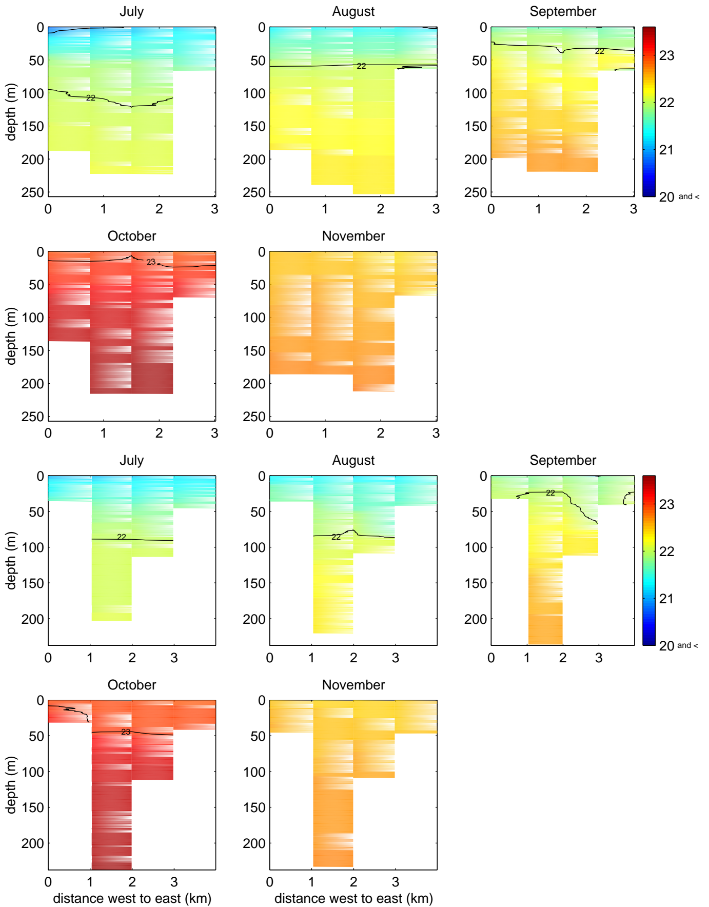
Figure 4–22. West Point (top 5 plots) and Alki (bottom 5 plots) Density (sigma-t) 2000
