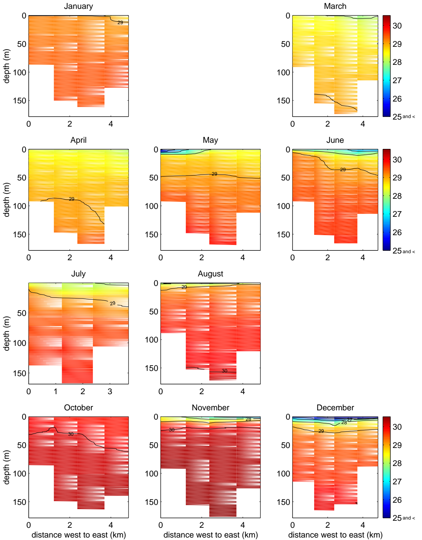
Figure 4–9. Point Wells Salinity (PSS) 1999
