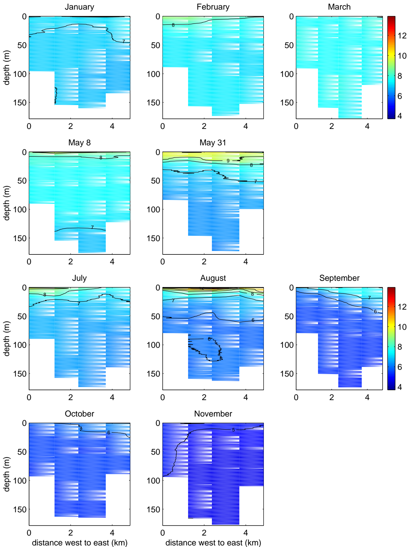
Figure 4-33. Point Wells Dissolved Oxygen (mg/L) 2000
