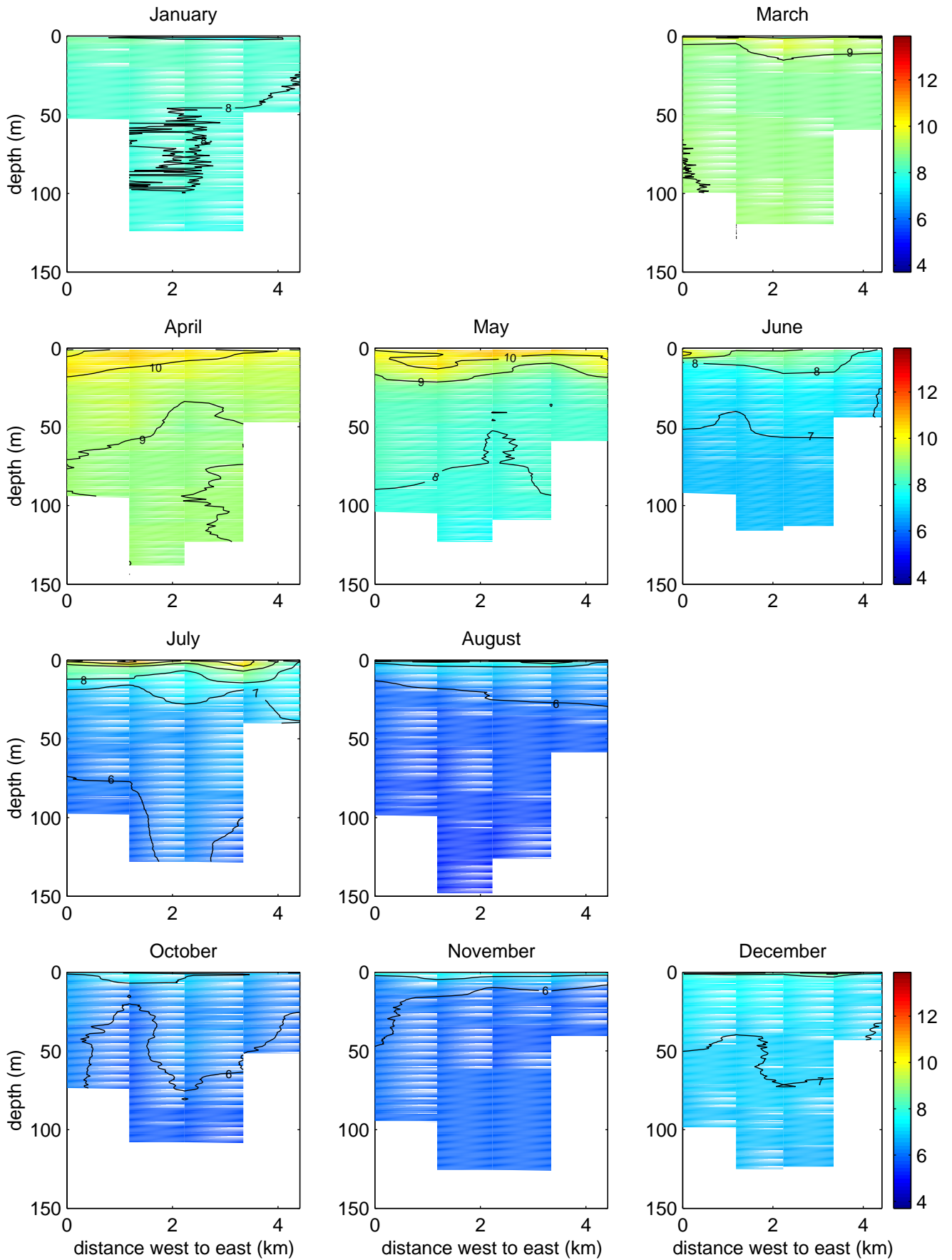
Figure 4–32. Admiralty Dissolved Oxygen (mg/L) 1999
